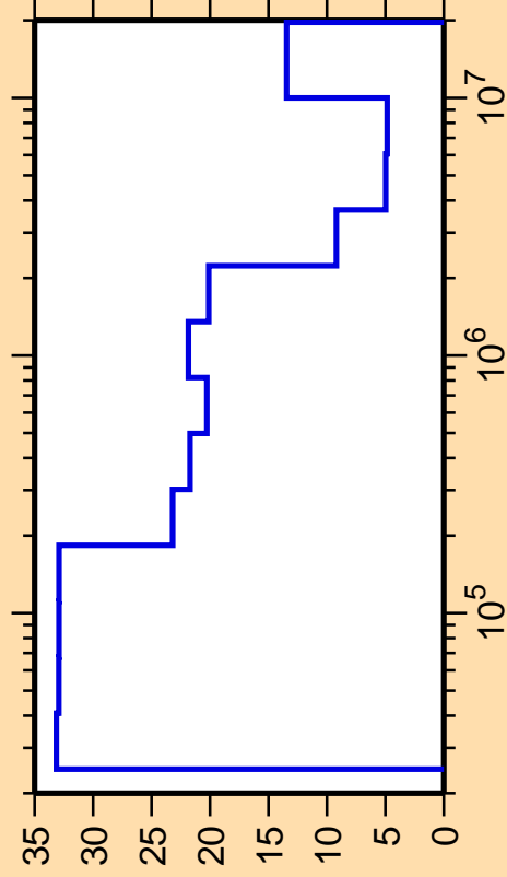
\Delta\sigma/\sigma vs. E for ^{120}\text{I}(n,\text{inel.})
