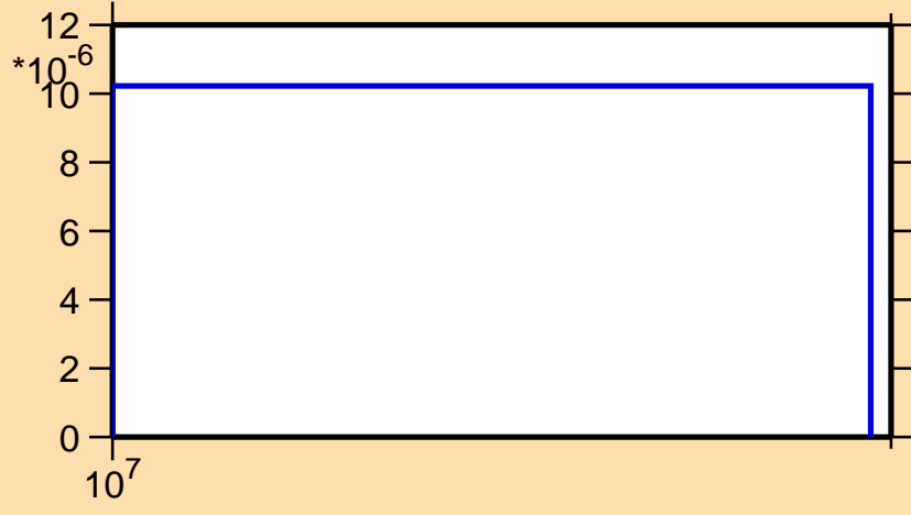
\sigma vs. E for ^{120}\text{I}(n,\text{nd})
