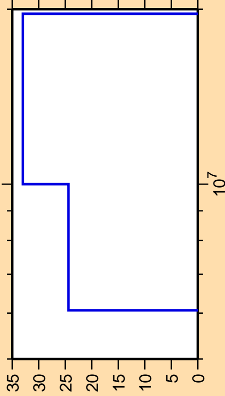
\Delta\sigma/\sigma vs. E for ^{120}\text{I}(n,n_1)
