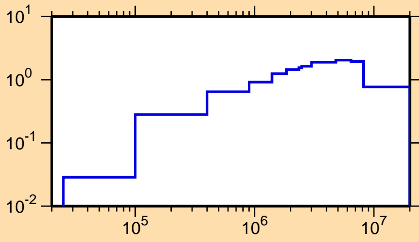
\sigma vs. E for ^{120}\text{I}(n,\text{inel.})
