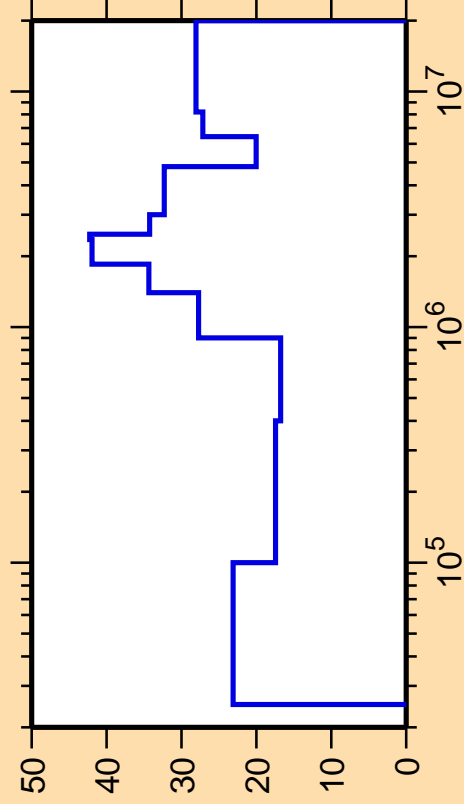
\Delta\sigma/\sigma vs. E for ^{120}\text{I}(n,n_2)
