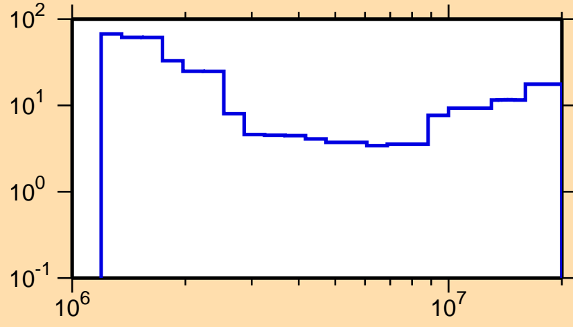
\Delta\sigma/\sigma vs. E for ^{121}\text{I}(n,ncont.)
