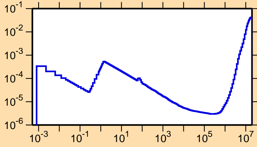
\sigma vs. E for ^{121}\text{I}(n,\alpha)
