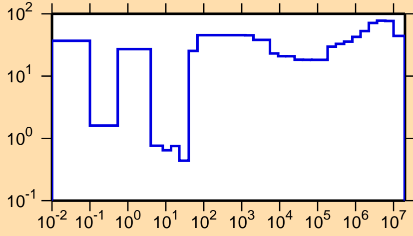
\Delta\sigma/\sigma vs. E for ^{121}\text{I}(n,\gamma)
