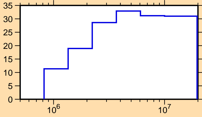
\Delta\sigma/\sigma vs. E for ^{121}\text{I}(n,n_1)
