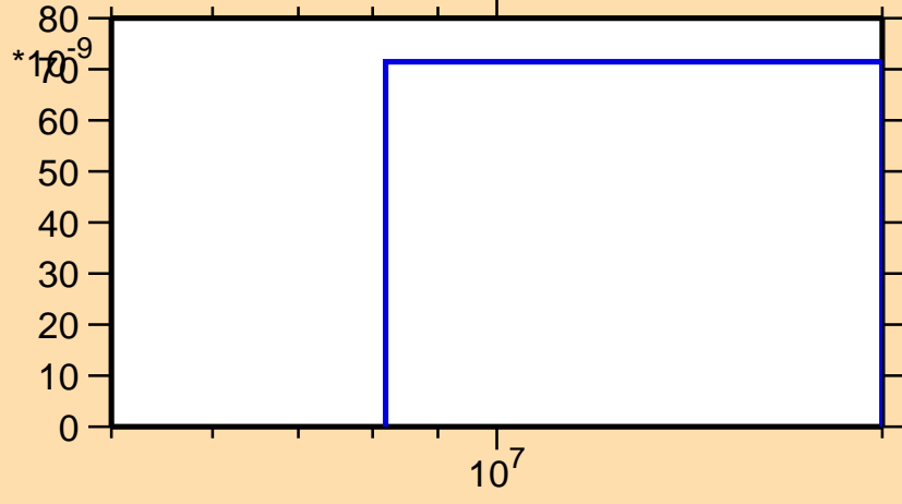
\sigma vs. E for ^{121}\text{I}(n,\text{nd})
