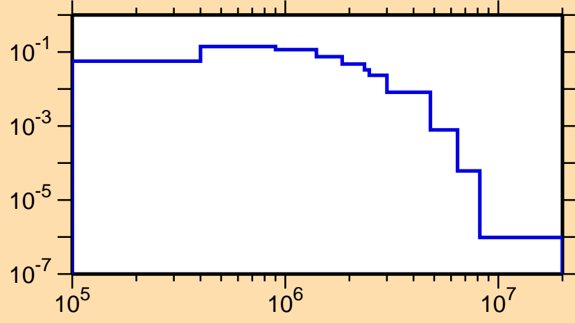
\sigma vs. E for ^{121}\text{I}(n,n_3)
