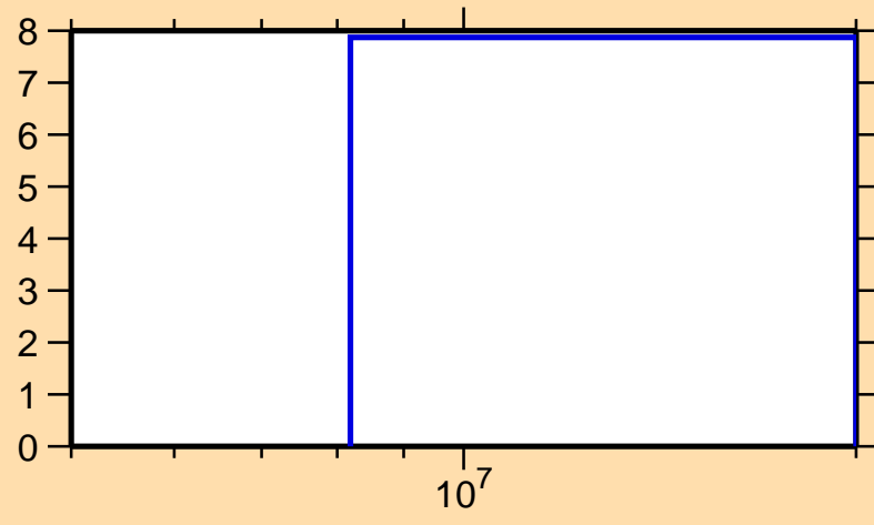
\Delta\sigma/\sigma vs. E for ^{121}\text{I}(n,\text{inel.})
