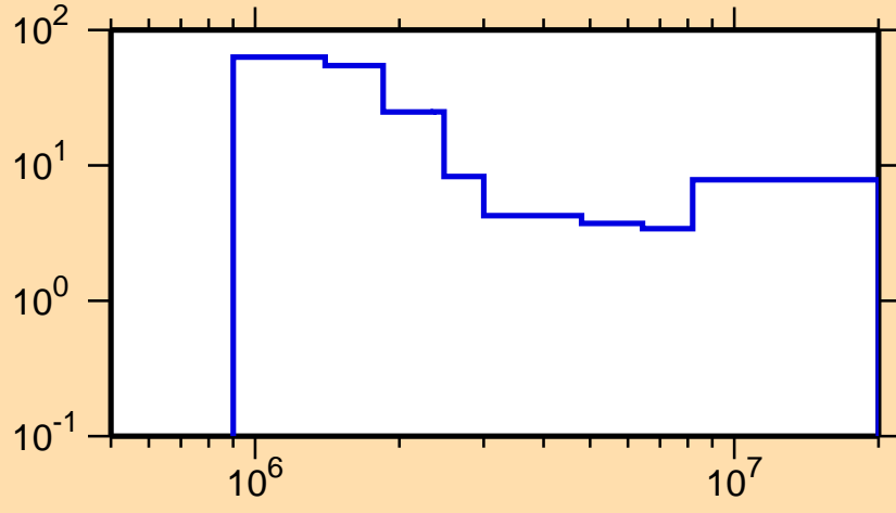
\Delta\sigma/\sigma vs. E for ^{121}\text{I}(n,n\text{cont.})
