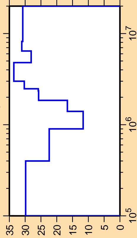
\Delta\sigma/\sigma vs. E for ^{121}\text{I}(n,n_3)
