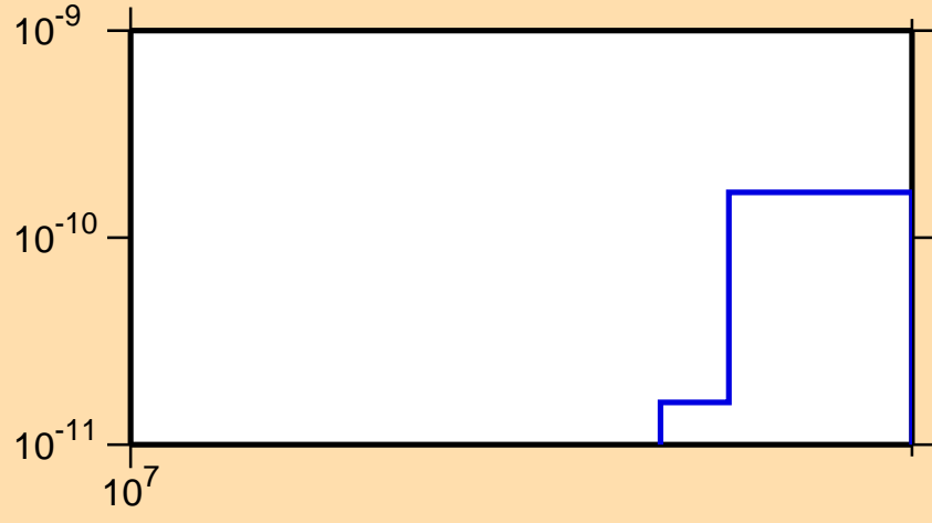
\sigma vs. E for ^{123}\text{I}(\text{mt117})
