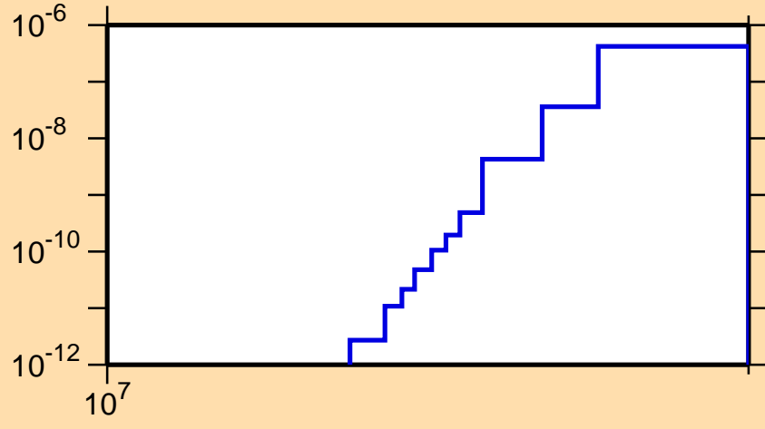
\sigma vs. E for ^{123}\text{I}(n,\text{He3})
