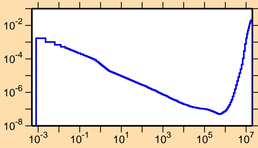
\sigma vs. E for ^{126}\text{I}(n,\alpha)
