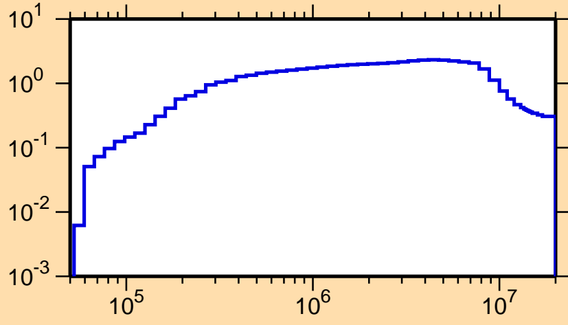
\sigma vs. E for ^{126}\text{I}(n,\text{inel.})
