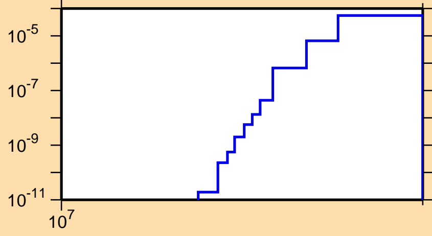
\sigma vs. E for ^{126}\text{I}(n,\text{nd})
