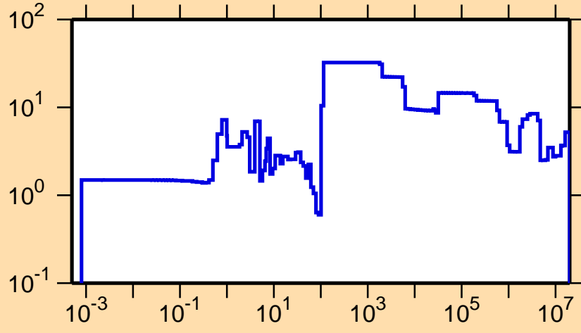
\Delta\sigma/\sigma vs. E for ^{126}\text{I}(n,el.)
