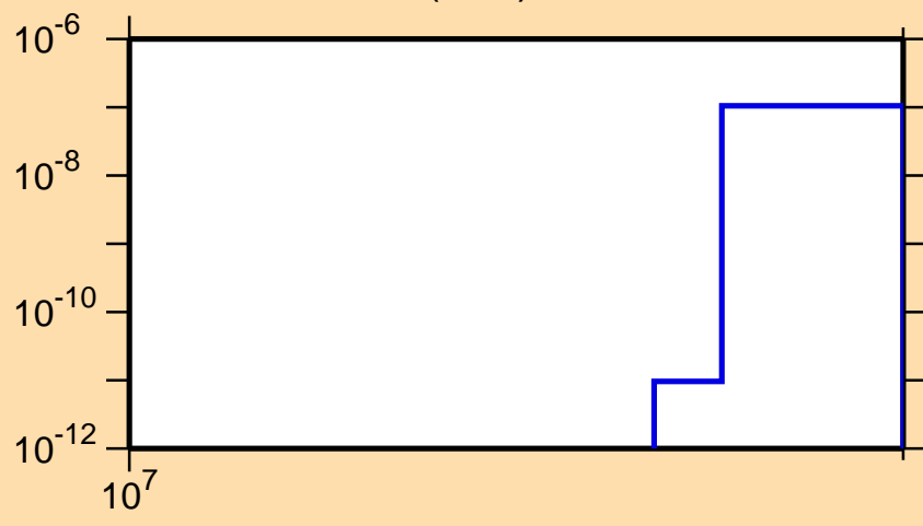
\sigma vs. E for ^{126}\text{I}(n,nt)
