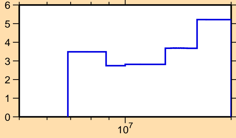
\Delta\sigma/\sigma vs. E for ^{126}\text{I}(n,\text{el.})
