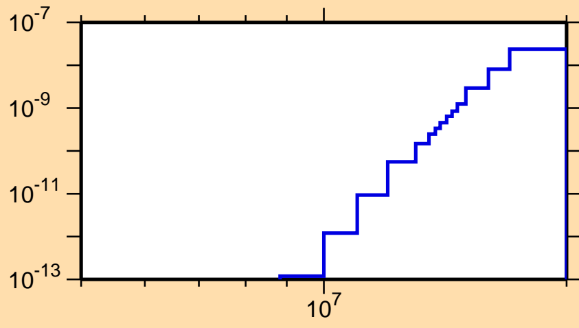
\sigma vs. E for ^{126}\text{I}(n,p\alpha)
