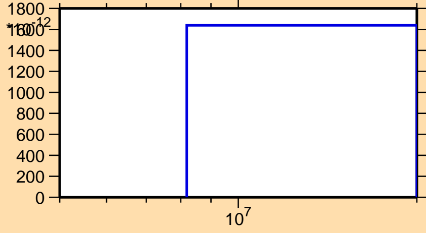
\sigma vs. E for ^{126}\text{I}(n,2n\alpha)
