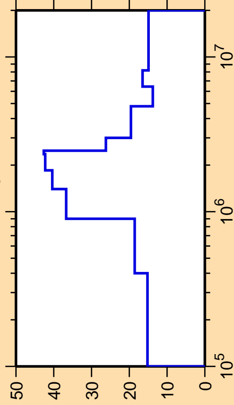
\Delta\sigma/\sigma vs. E for ^{126}\text{I}(n,n_3)
