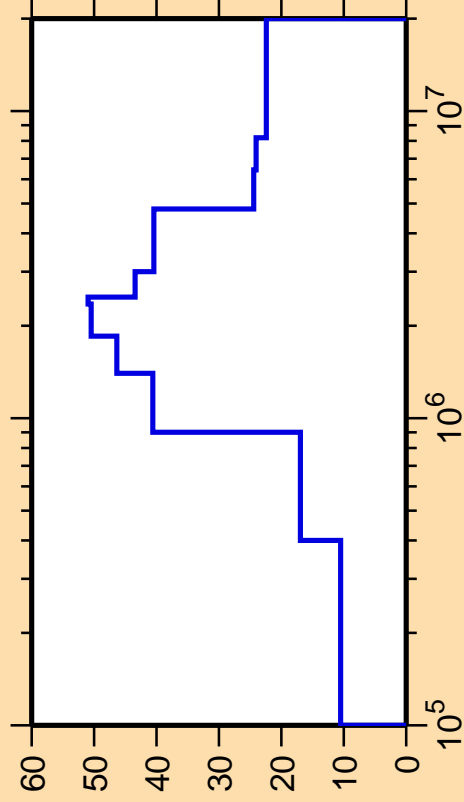
\Delta\sigma/\sigma vs. E for ^{126}\text{I}(n,n_2)
