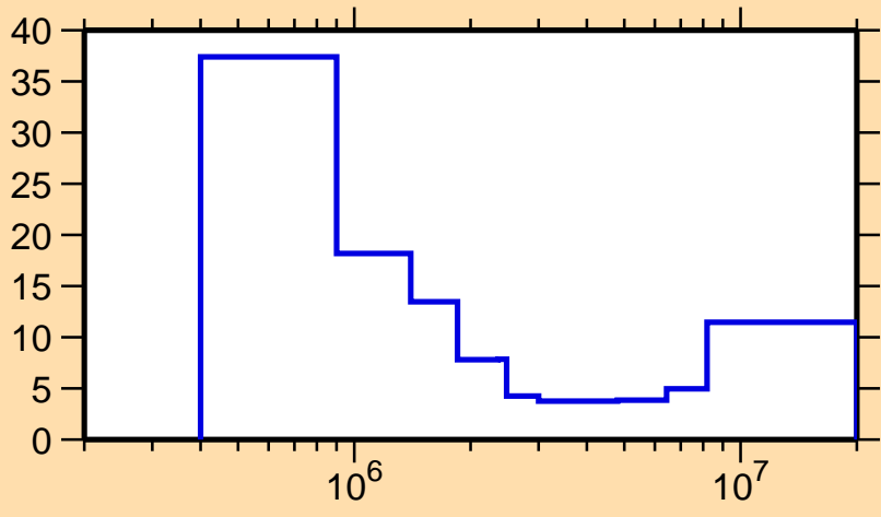
\Delta\sigma/\sigma vs. E for ^{126}\text{I}(n,ncont.)
