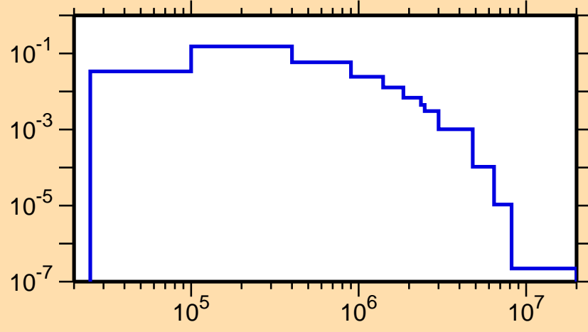
\sigma vs. E for ^{126}\text{I}(n,n_1)
