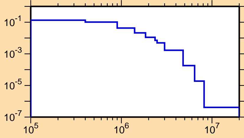
\sigma vs. E for ^{126}\text{I}(n,n_2)
