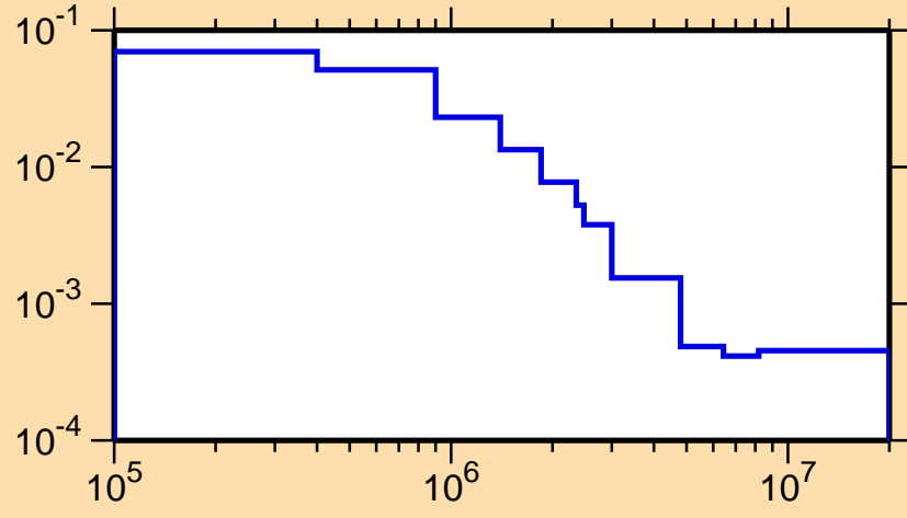
\sigma vs. E for ^{126}\text{I}(n,n_3)
