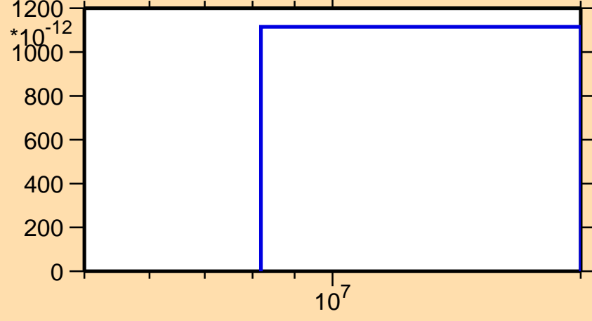
\sigma vs. E for ^{126}\text{I}(n,p\alpha)
