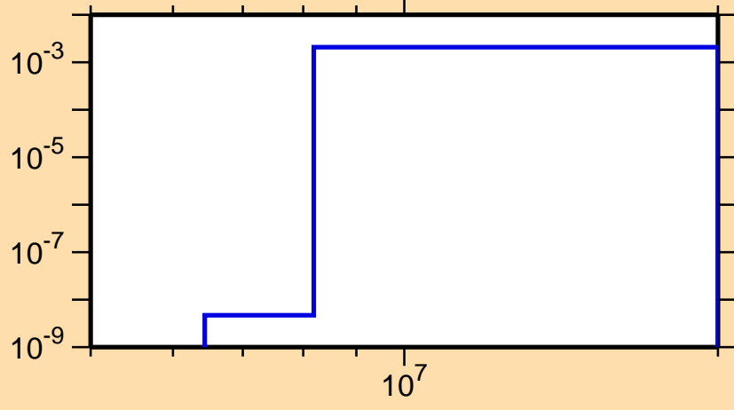
\sigma vs. E for ^{126}\text{I}(n,d)
