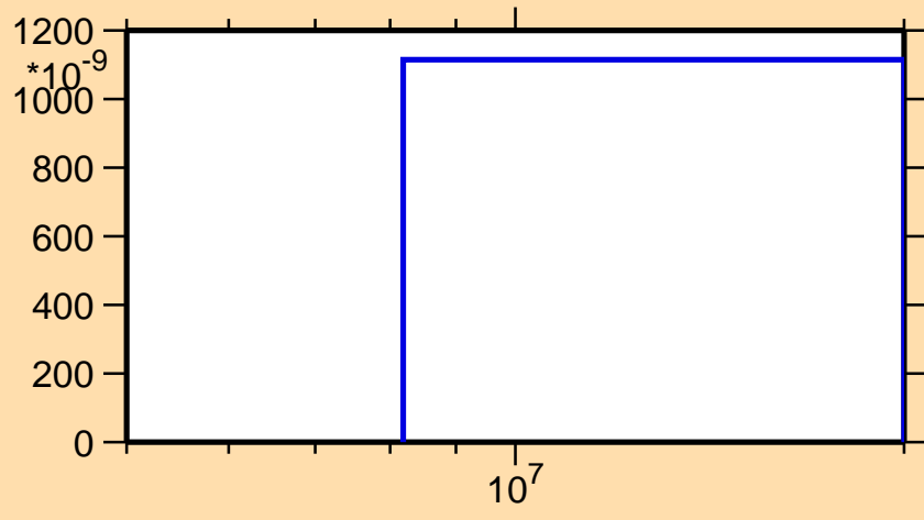
\sigma vs. E for ^{126}\text{I}(n,2np)
