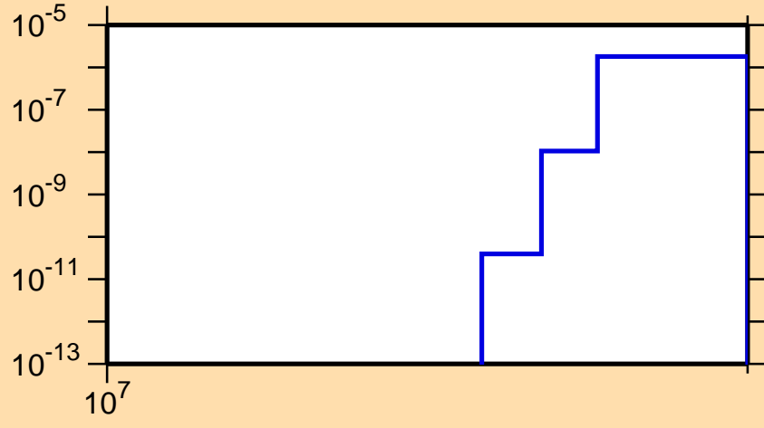
\sigma vs. E for ^{127}\text{I}(n,\text{nd})
