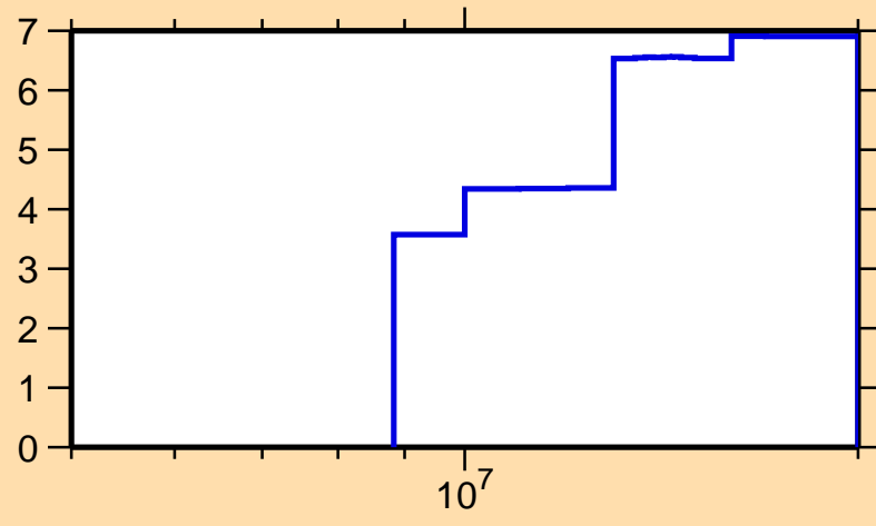
\Delta\sigma/\sigma vs. E for ^{127}\text{I}(n,\text{inel.})
