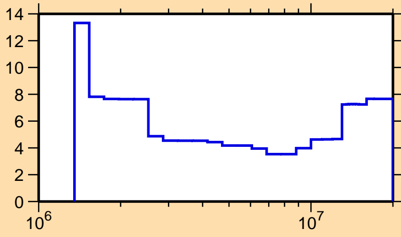
\Delta\sigma/\sigma vs. E for ^{127}\text{I}(n,ncont.)
