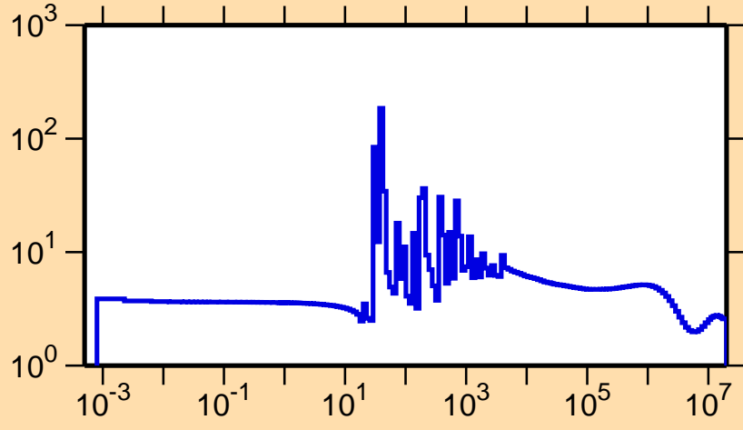
\sigma vs. E for ^{127}\text{I}(n,\text{el.})
