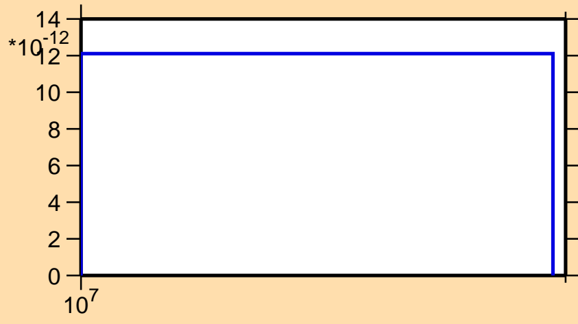
\sigma vs. E for ^{127}\text{I}(n,p\alpha)
