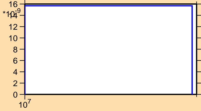
\sigma vs. E for ^{127}\text{I}(n,nd)
