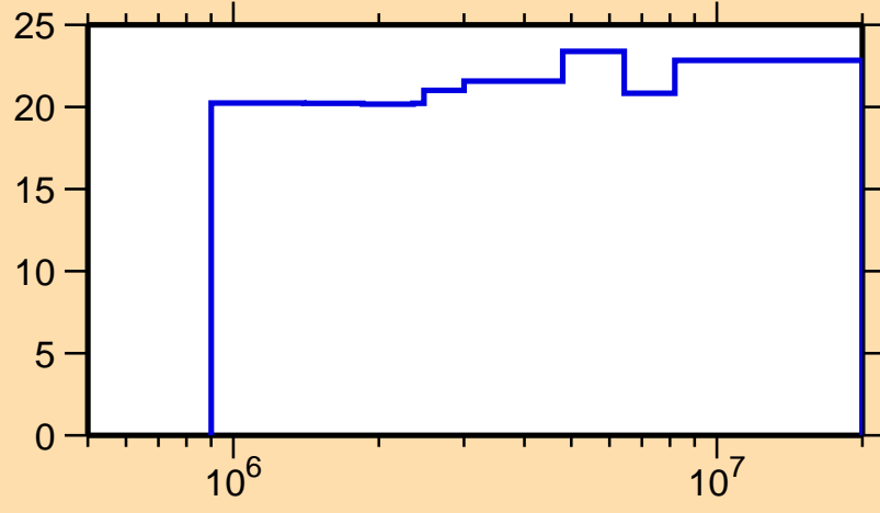
\Delta\sigma/\sigma vs. E for ^{127}\text{I}(n,\gamma)
