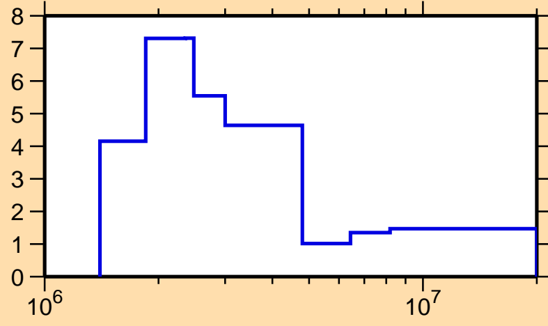
\Delta\sigma/\sigma vs. E for ^{127}\text{I}(n, tot.)
