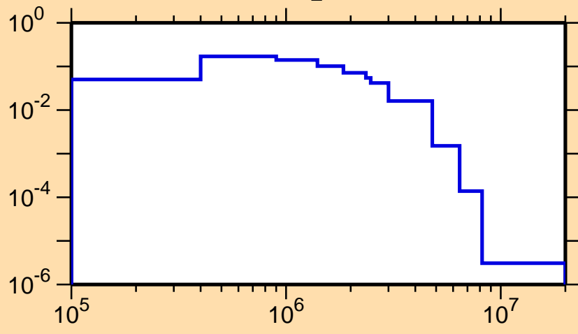
\sigma vs. E for ^{127}\text{I}(n,n_2)
