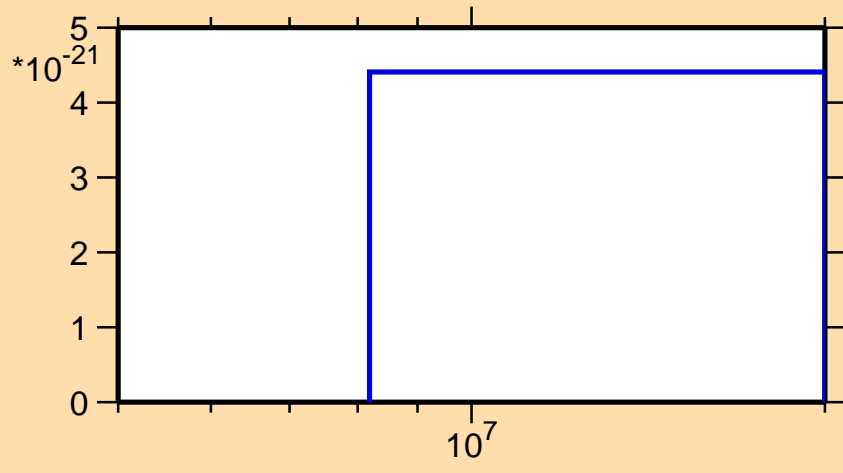
\sigma vs. E for ^{127}\text{I} (mt 11)
