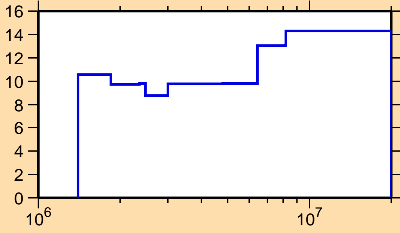
\Delta\sigma/\sigma vs. E for ^{127}\text{I}(n,n_1)
