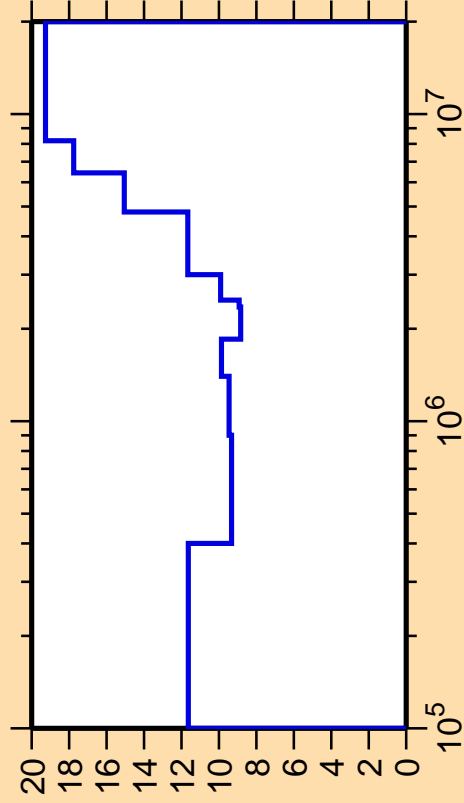
\Delta\sigma/\sigma vs. E for ^{127}\text{I}(n,n_2)
