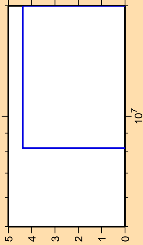
\Delta\sigma/\sigma vs. E for ^{127}\text{I}(n,n\text{cont.})
