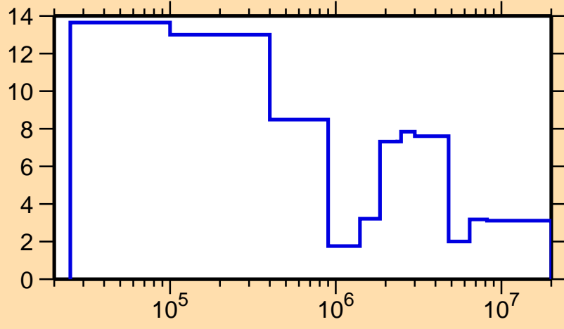
\Delta\sigma/\sigma vs. E for ^{127}\text{I}(n,\text{el.})
