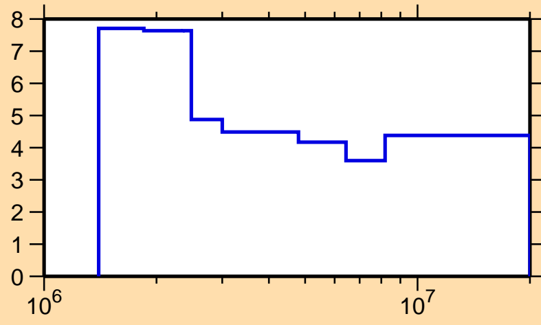
\Delta\sigma/\sigma vs. E for ^{127}\text{I}(n,n\text{cont.})
