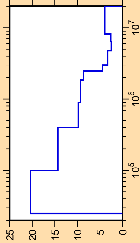
\Delta\sigma/\sigma vs. E for ^{127}\text{I}(n,\text{inel.})
