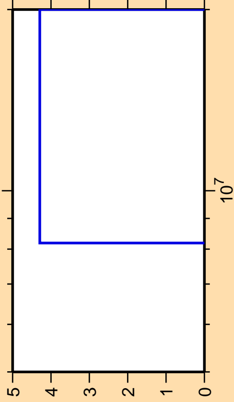
\Delta\sigma/\sigma vs. E for ^{127}\text{I}(n,2n)
