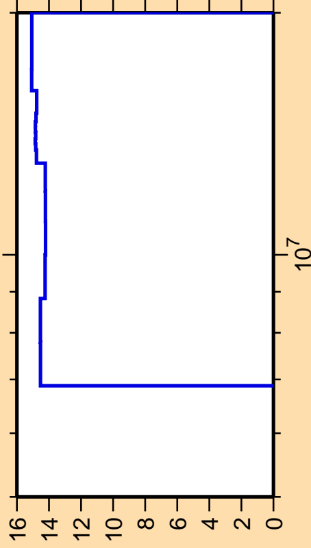
\Delta\sigma/\sigma vs. E for ^{128}\text{I}(n,n_1)
