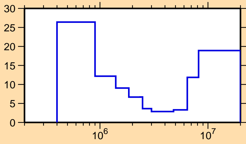
\Delta\sigma/\sigma vs. E for ^{128}\text{I}(n,n\text{cont.})
