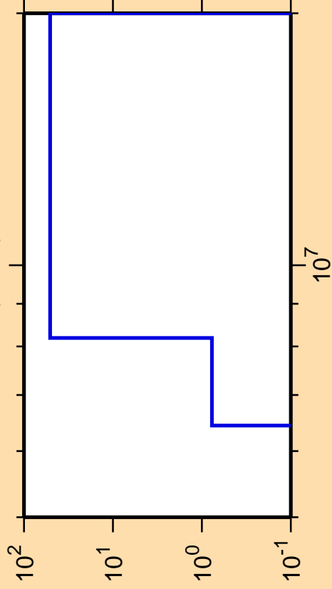
\Delta\sigma/\sigma vs. E for ^{128}\text{I}(n,n\alpha)
