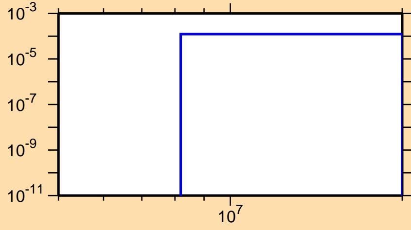
\sigma vs. E for ^{128}\text{I}(n,n\alpha)
