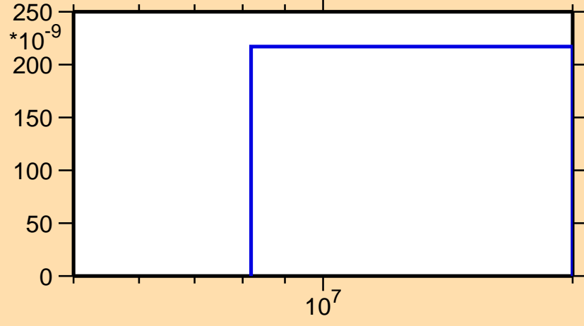
\sigma vs. E for ^{130}\text{I}(n,nd)
