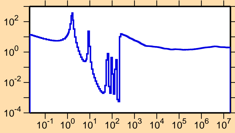
\sigma vs. E for ^{130}\text{I}(n,\text{nonel.})
