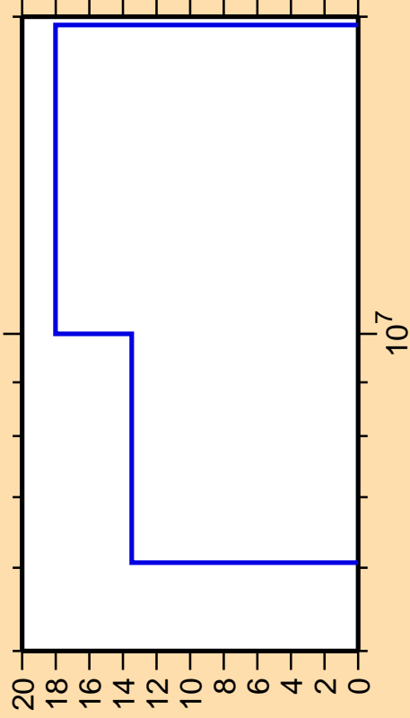
\Delta\sigma/\sigma vs. E for ^{130}\text{I}(n,p)
