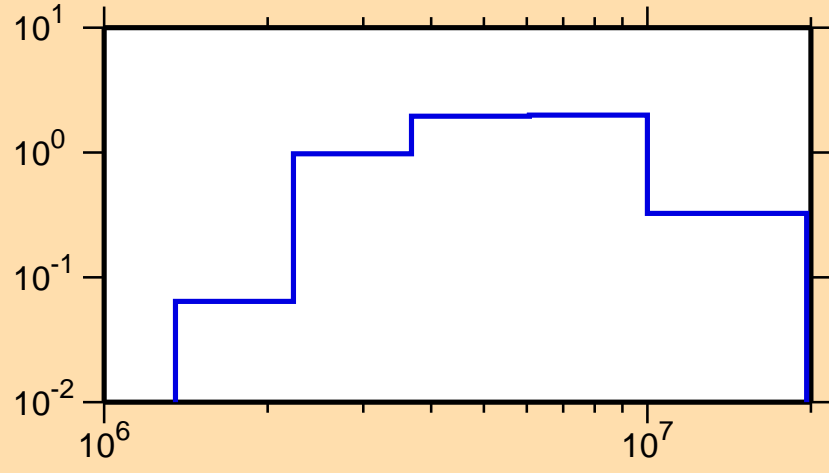
\sigma vs. E for ^{131}\text{I}(n,n\text{cont.})
