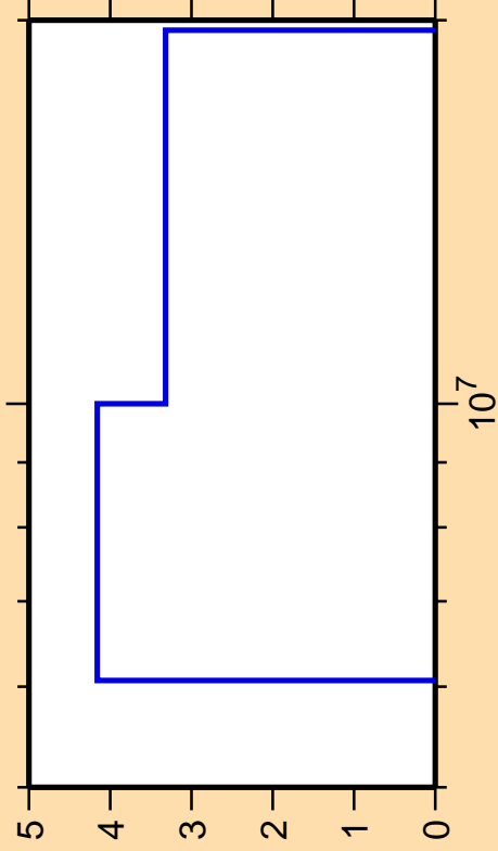
\Delta\sigma/\sigma vs. E for ^{131}\text{I}(n,2n)
