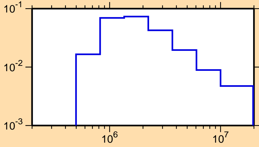
\sigma vs. E for ^{131}\text{I}(n,n_3)
