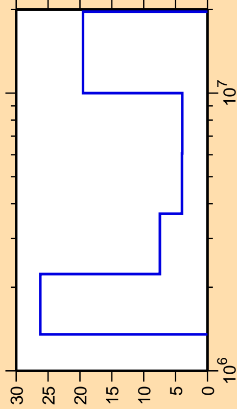
\Delta\sigma/\sigma vs. E for ^{131}\text{I}(n,n\text{cont.})
