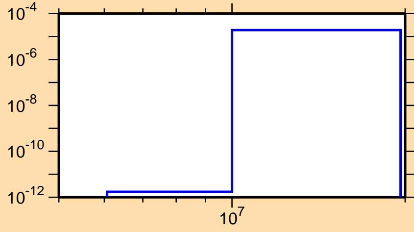
\sigma vs. E for ^{131}\text{I}(n,n\alpha)
