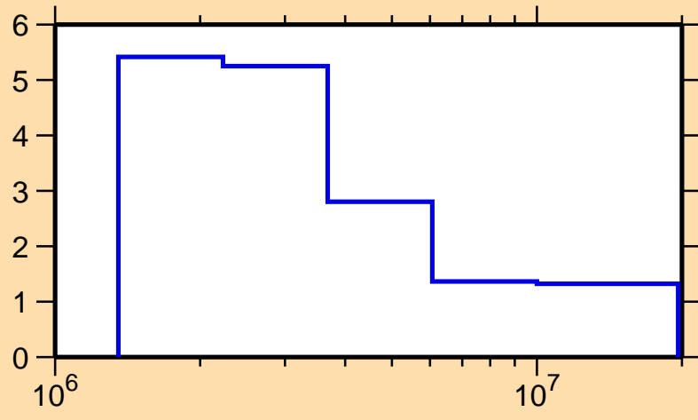
\Delta\sigma/\sigma vs. E for ^{131}\text{I}(n, tot.)
