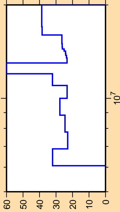
\Delta\sigma/\sigma vs. E for ^{132}\text{I}(n,n_1)
