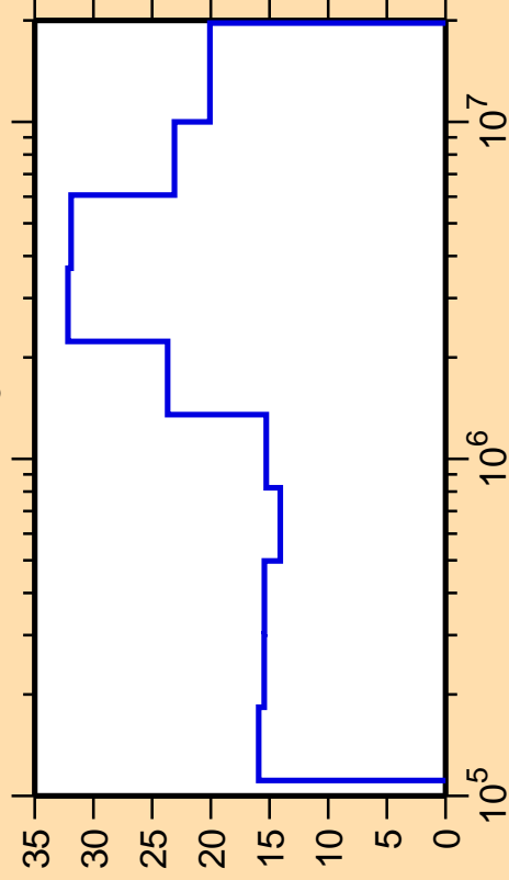
\Delta\sigma/\sigma vs. E for ^{132}\text{I}(n,n_3)
