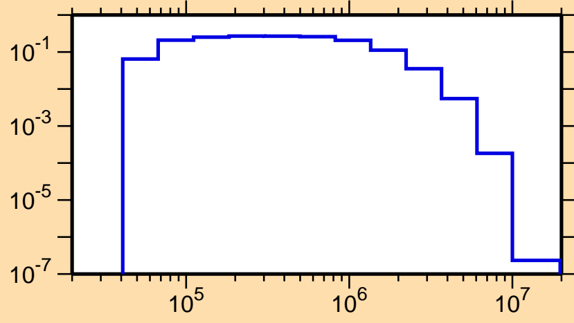
\sigma vs. E for ^{132}\text{I}(n,n_2)
