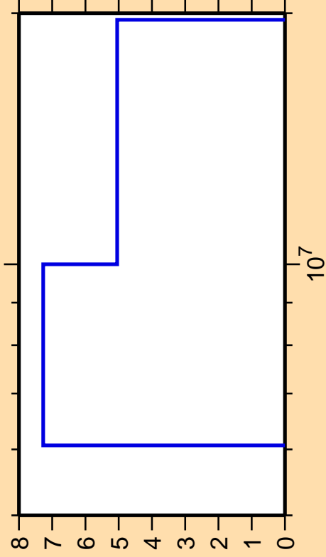
\Delta\sigma/\sigma vs. E for ^{132}\text{I}(n,2n)
