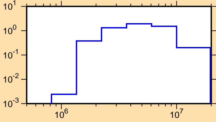
\sigma vs. E for ^{132}\text{I}(n,n\text{cont.})
