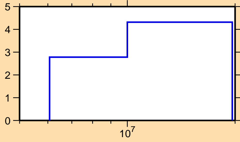
\Delta\sigma/\sigma vs. E for ^{132}\text{I}(n,\text{el.})
