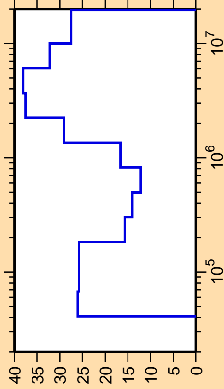
\Delta\sigma/\sigma vs. E for ^{132}\text{I}(n,n_2)
