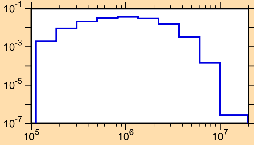
\sigma vs. E for ^{132}\text{I}(n,n_3)
