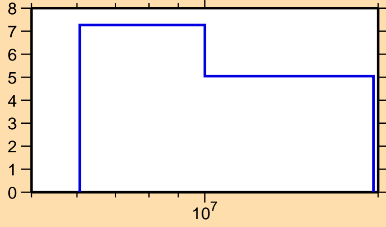
\Delta\sigma/\sigma vs. E for ^{132}\text{I}(n,2n)
