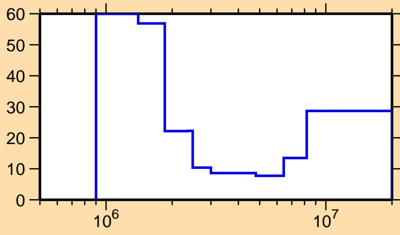
\Delta\sigma/\sigma vs. E for ^{132}\text{I}(n,n\text{cont.})
