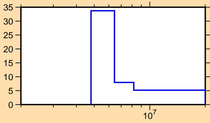
\Delta\sigma/\sigma vs. E for ^{132}\text{I}(n,2n)
