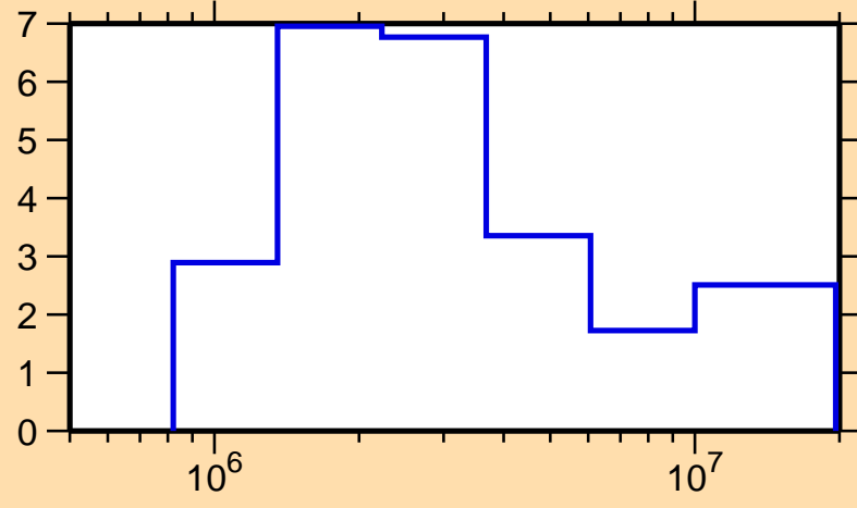
\Delta\sigma/\sigma vs. E for ^{132}\text{I}(n, tot.)
