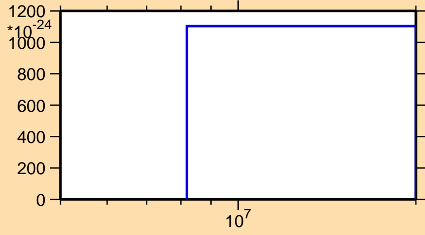
\sigma vs. E for ^{132}\text{I}(\text{mt } 11)
