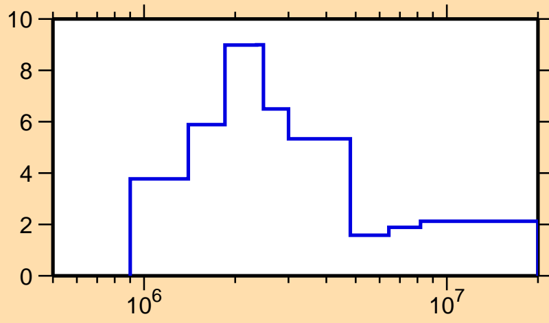
\Delta\sigma/\sigma vs. E for ^{132}\text{I}(n, tot.)
