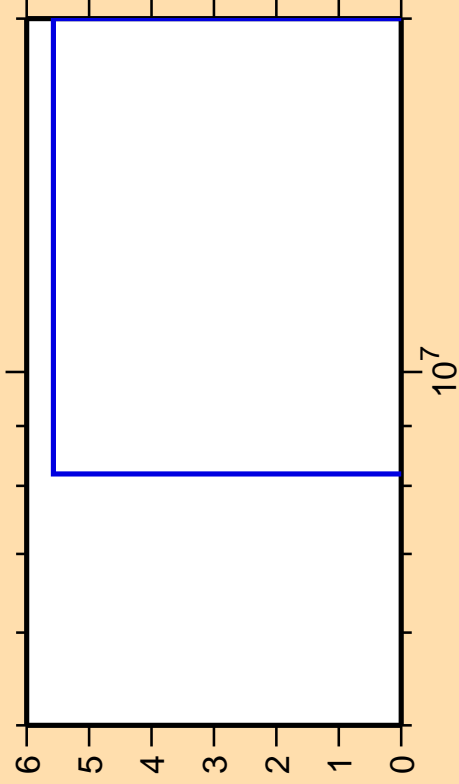
\Delta\sigma/\sigma vs. E for ^{133}\text{I}(n,2n\alpha)
