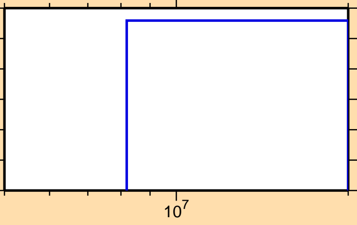
\sigma vs. E for ^{133}\text{I}(n,3n)
