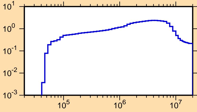
\sigma vs. E for ^{134}\text{I}(n,\text{inel.})
