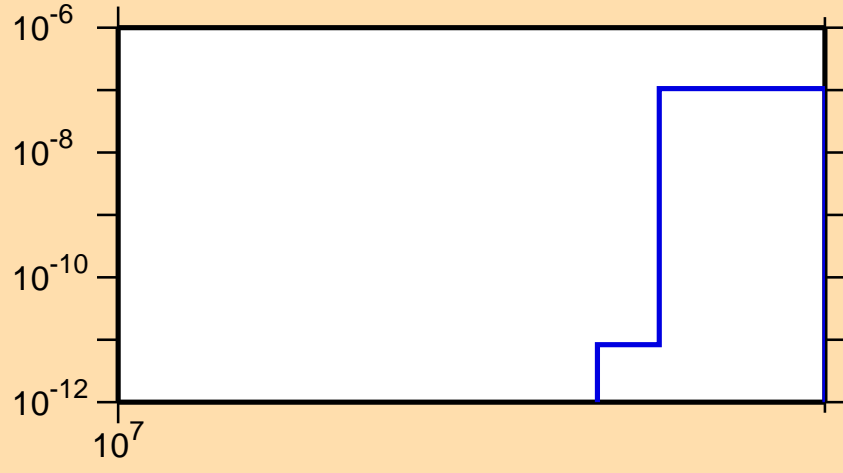
\sigma vs. E for ^{134}\text{I}(n,nt)
