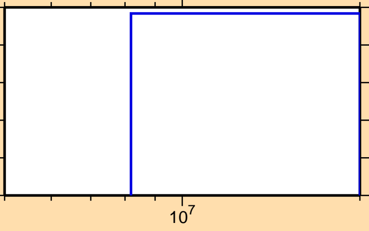
\sigma vs. E for ^{134}\text{I}(n,n\alpha)
