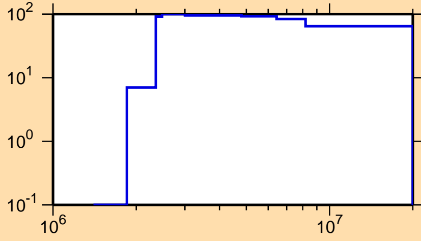
\Delta\sigma/\sigma vs. E for ^{134}\text{I}(n,p)
