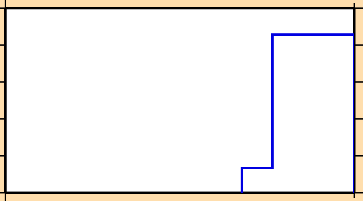
\sigma vs. E for ^{134}\text{I}(n,nt)
