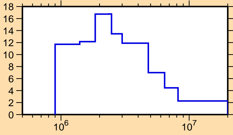
\Delta\sigma/\sigma vs. E for ^{134}\text{I}(n, tot.)
