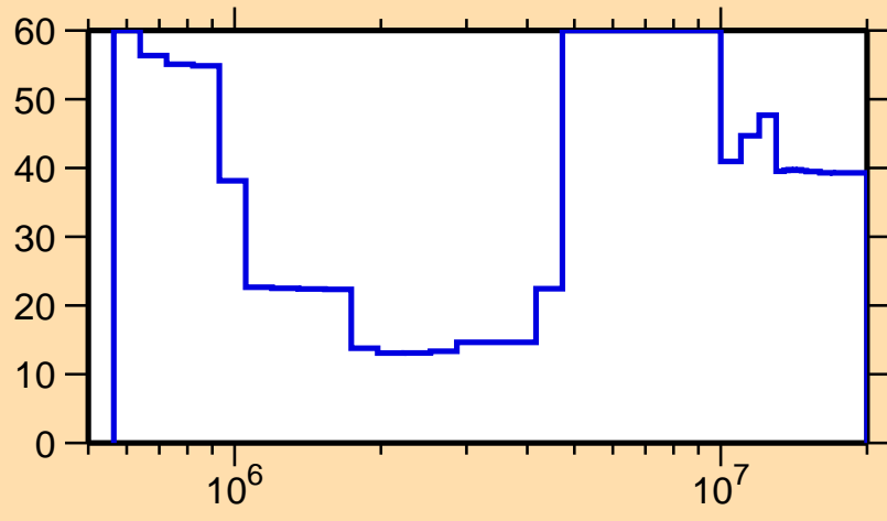
\Delta\sigma/\sigma vs. E for ^{135}\text{I}(n,n_1)
