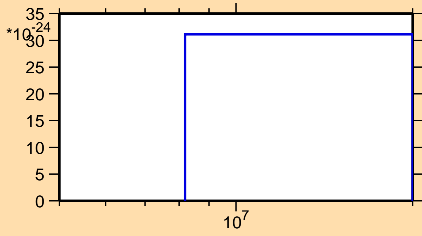
\sigma vs. E for ^{135}\text{I} (mt 11)
