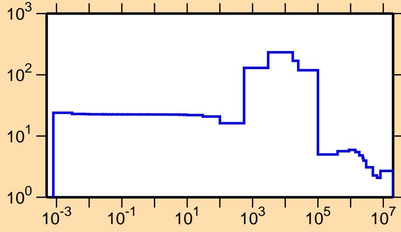
\sigma vs. E for ^{135}\text{I}(n,\text{el.})
