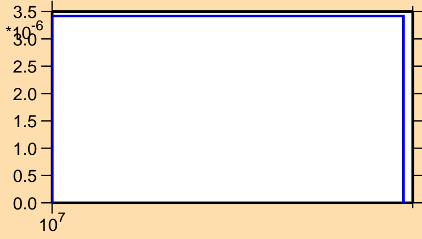
\sigma vs. E for ^{136}\text{I}(n,\text{nd})
