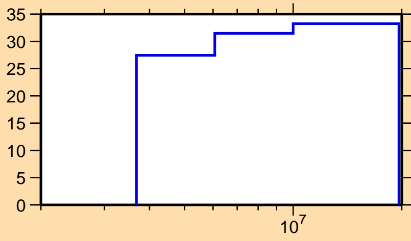
\Delta\sigma/\sigma vs. E for ^{136}\text{I}(n,ncont.)
