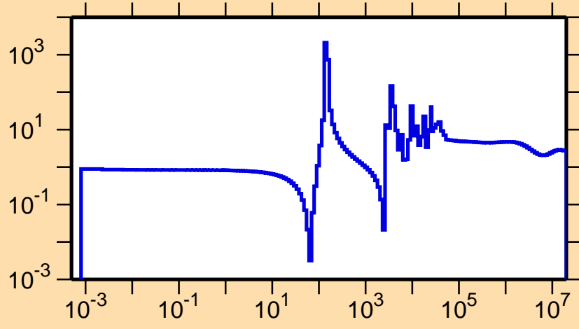
\sigma vs. E for ^{138}\text{I}(n,\text{el.})
