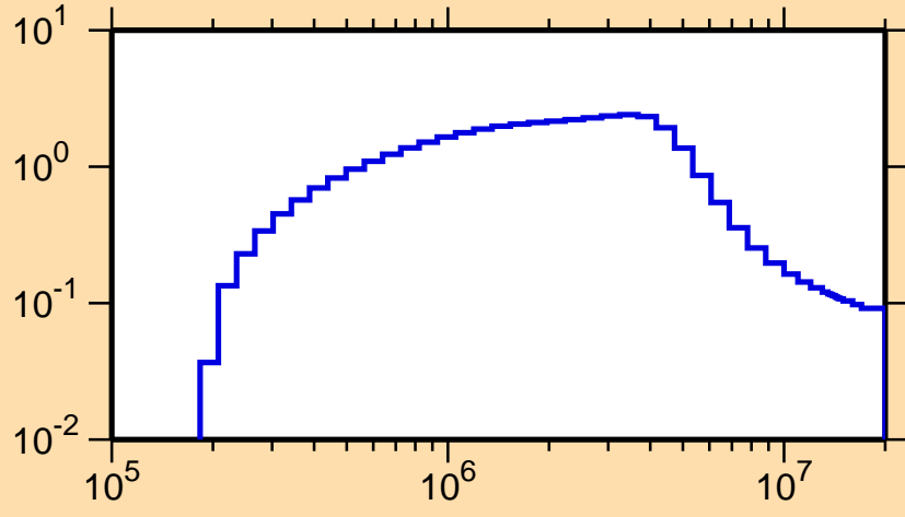
\sigma vs. E for ^{138}\text{I}(n,\text{inel.})
