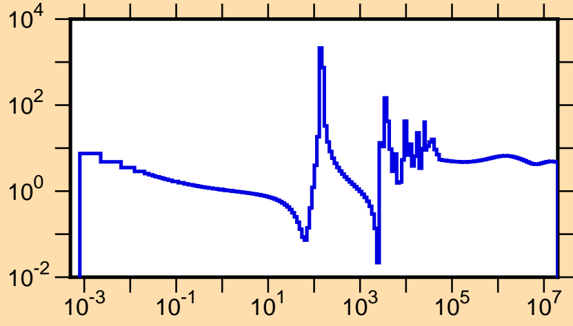
\sigma vs. E for ^{138}\text{I}(n,\text{tot.})
