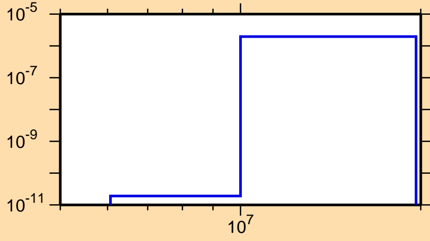
\sigma vs. E for ^{138}\text{I}(n,2n\alpha)
