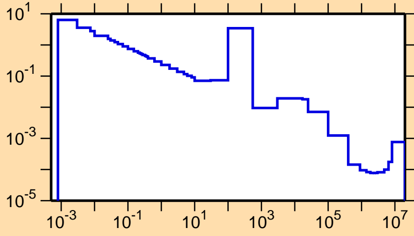
\sigma vs. E for ^{138}\text{I}(n,\gamma)
