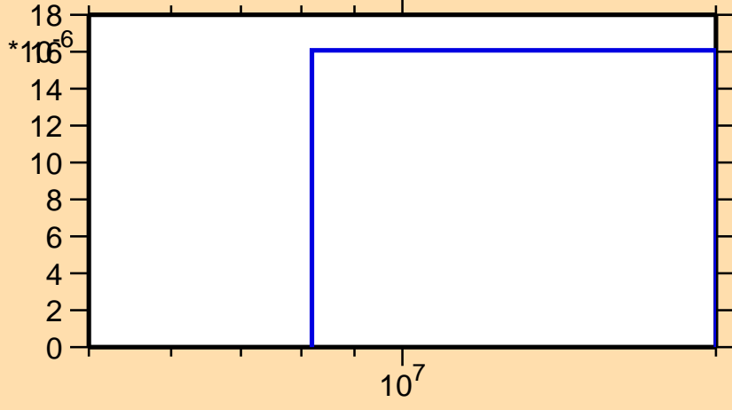
\sigma vs. E for ^{138}\text{I}(n,np)
