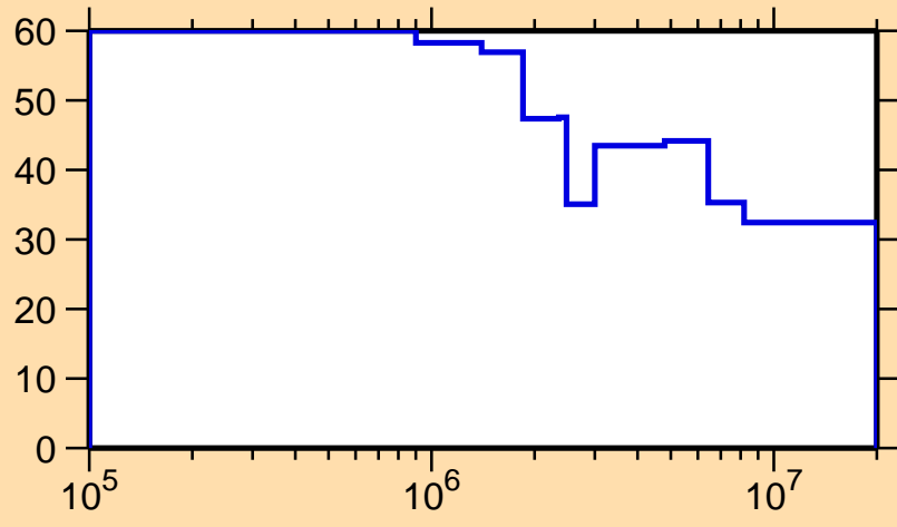
\Delta\sigma/\sigma vs. E for ^{138}\text{I}(n,n_1)
