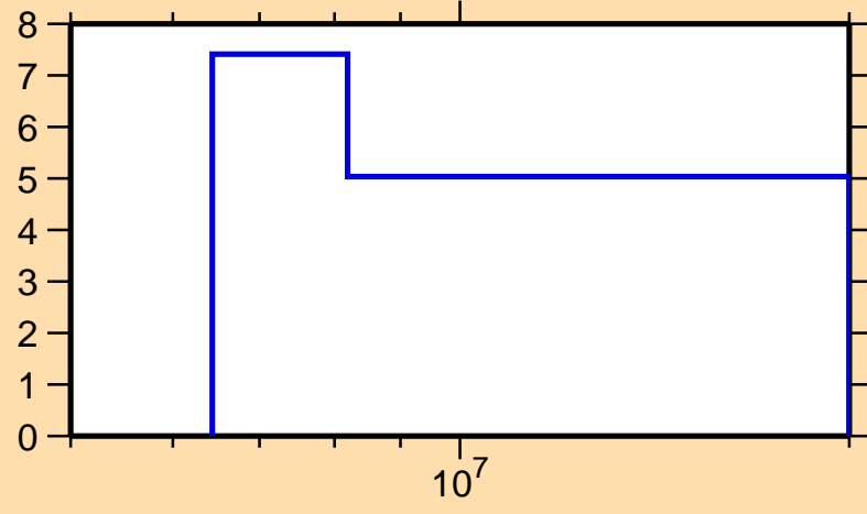
\Delta\sigma/\sigma vs. E for ^{138}\text{I}(n,\text{tot.})
