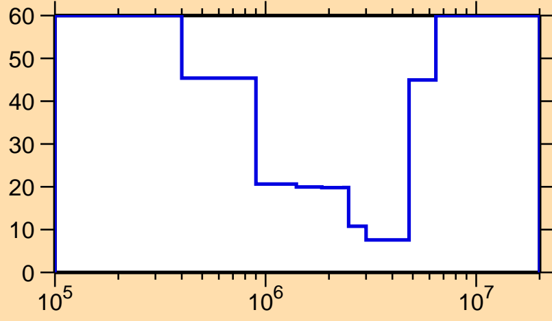
\Delta\sigma/\sigma vs. E for ^{138}\text{I}(n,n\text{cont.})
