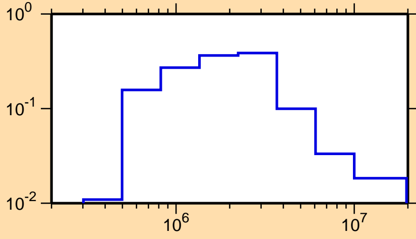
\sigma vs. E for ^{139}\text{I}(n,n_3)
