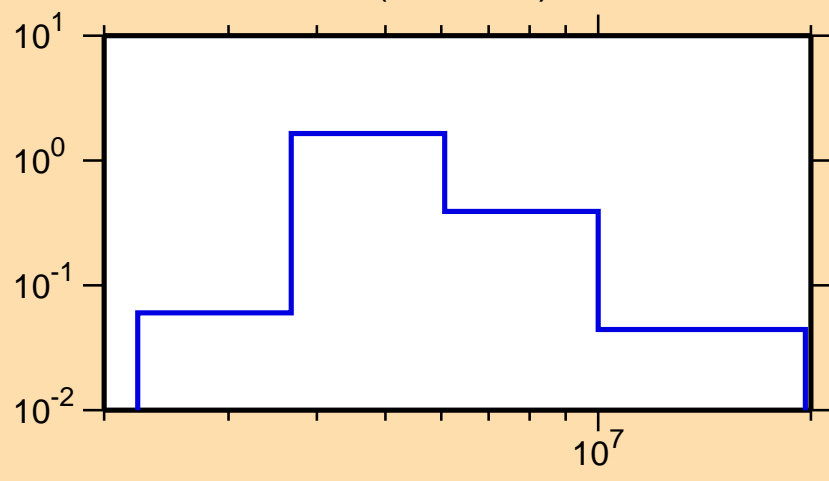
\sigma vs. E for ^{139}\text{I}(n,n\text{cont.})
