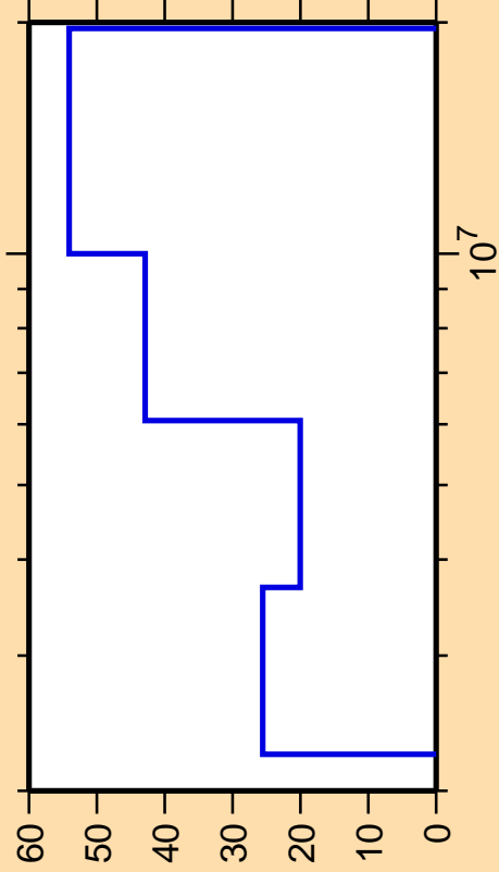
\Delta\sigma/\sigma vs. E for ^{139}\text{I}(n,n\text{cont.})
