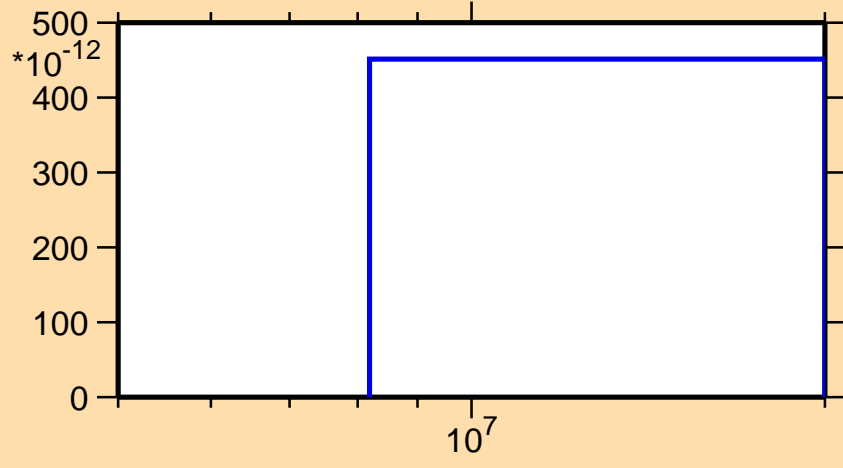
\sigma vs. E for ^{139}\text{I}(n,2np)
