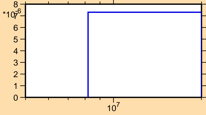
\sigma vs. E for ^{139}\text{I}(n,np)
