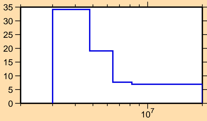
\Delta\sigma/\sigma vs. E for ^{139}\text{I}(n,\text{el.})
