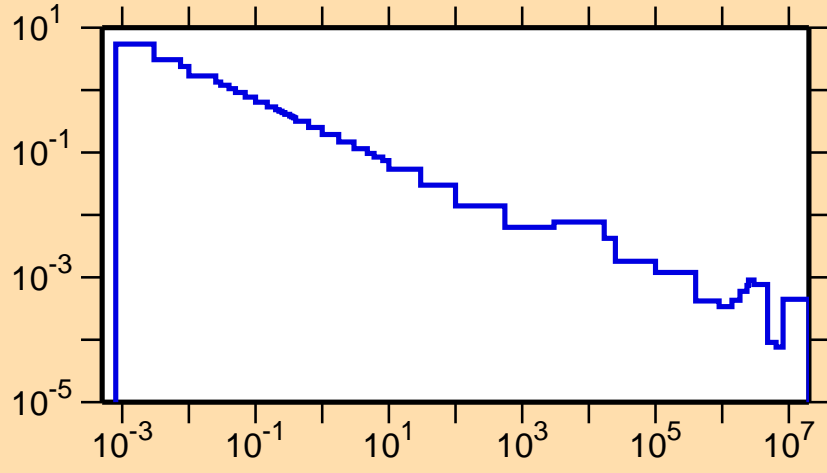
\sigma vs. E for ^{139}\text{I}(n,\gamma)
