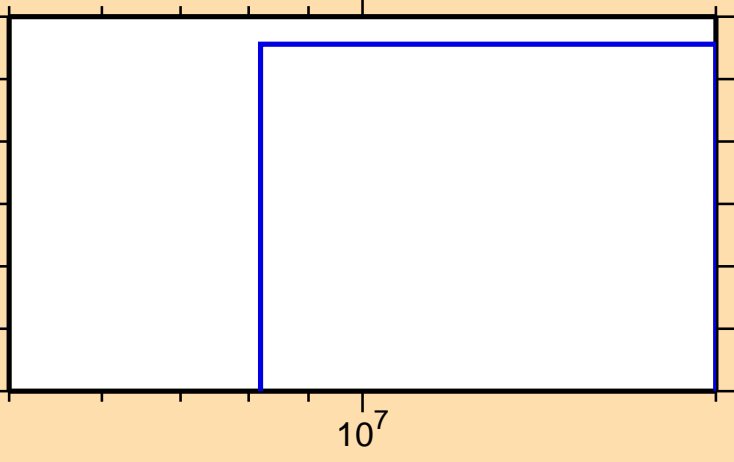
\sigma vs. E for ^{139}\text{I}(n,\text{nd})
