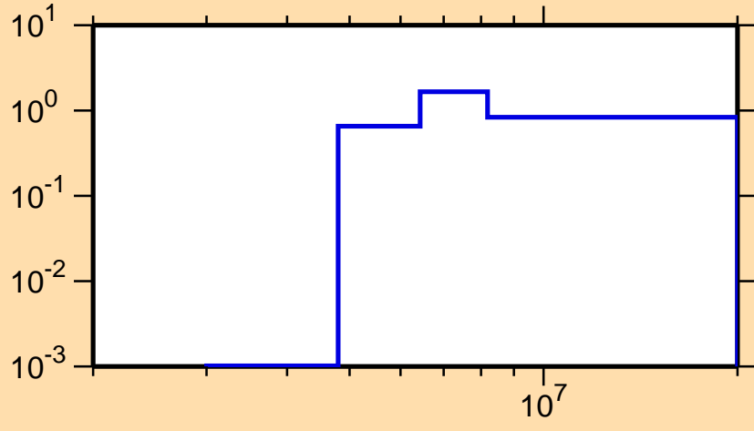
\sigma vs. E for ^{139}\text{I}(n,2n)
