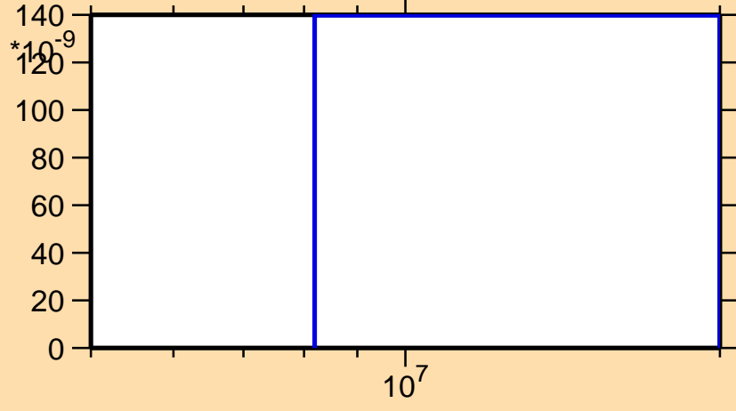
\sigma vs. E for ^{139}\text{I}(n,2n\alpha)
