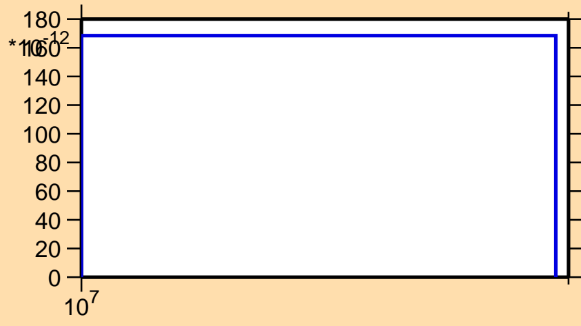
\sigma vs. E for ^{98}\text{In}(\text{mt } 45)
