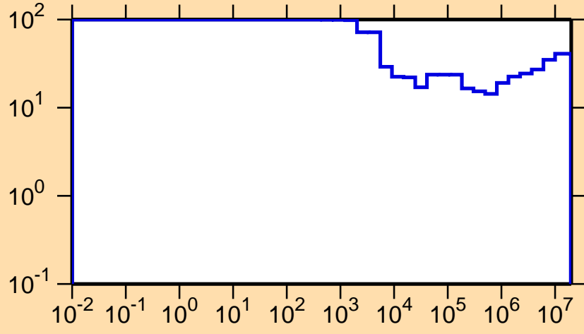
\Delta\sigma/\sigma vs. E for ^{98}\text{In}(n,p)
