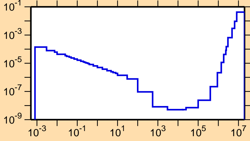
\sigma vs. E for ^{98}\text{In}(n,d)
