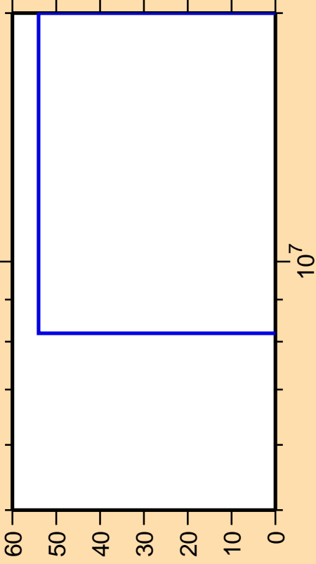
\Delta\sigma/\sigma vs. E for ^{98}\text{In}(n,2n)
