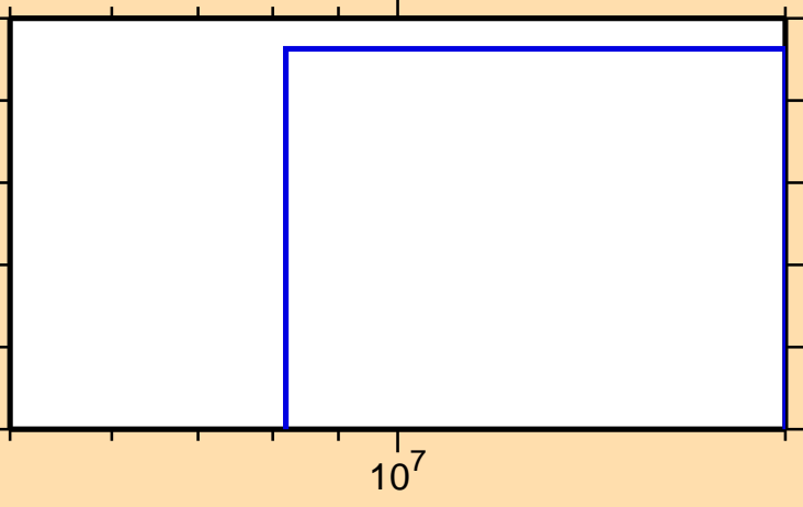
\sigma vs. E for ^{98}\text{In}(n,\text{nd})
