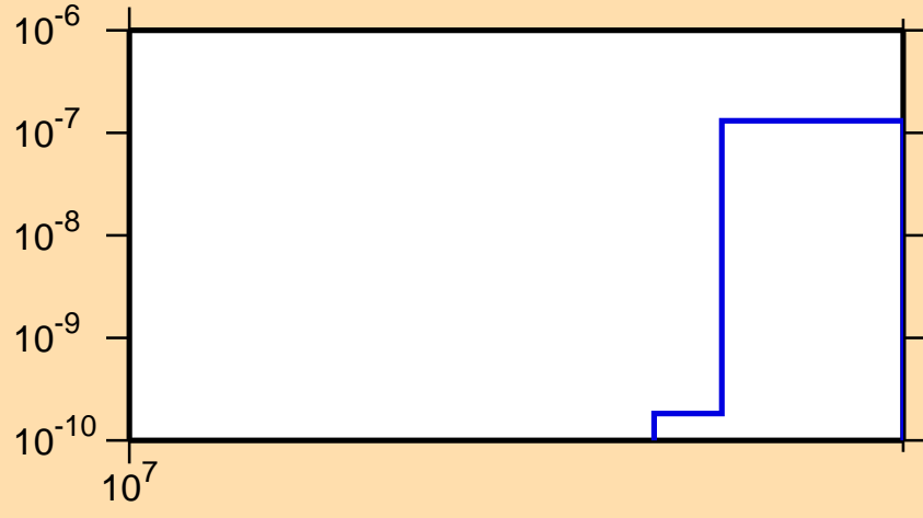
\sigma vs. E for ^{99}\text{In}(n,\text{nd})
