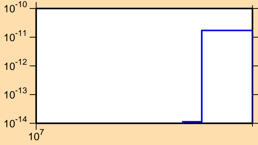
\sigma vs. E for ^{99}\text{In} (mt 34)
