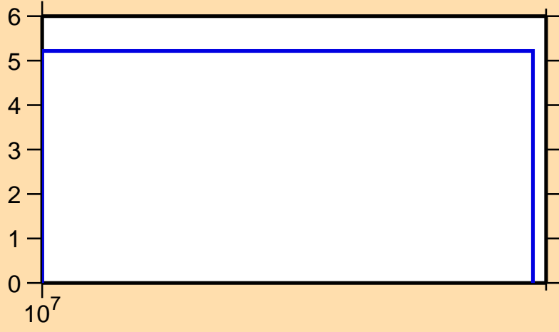
\Delta\sigma/\sigma vs. E for ^{99}\text{In}(n,\text{tot.})
