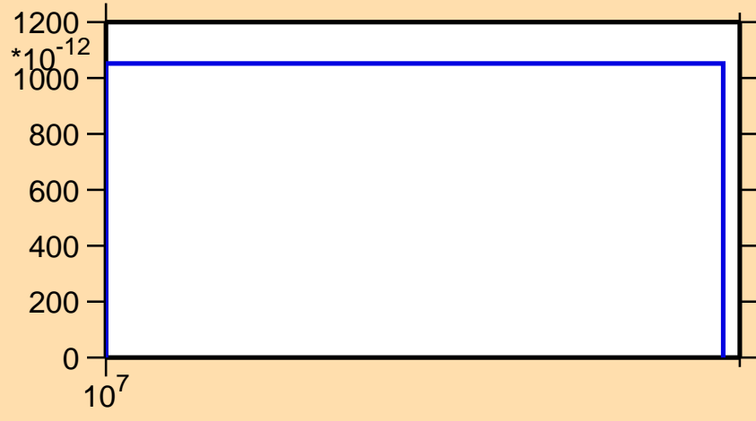
\sigma vs. E for ^{99}\text{In}(n,nd)
