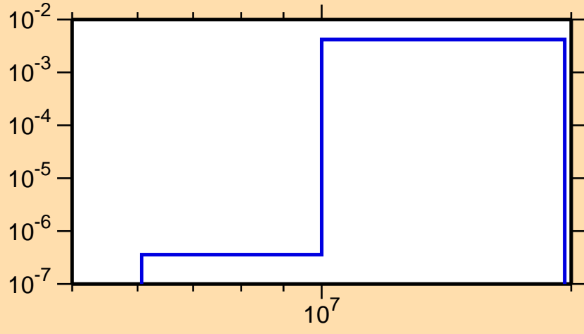
\sigma vs. E for ^{99}\text{In}(n,pd)
