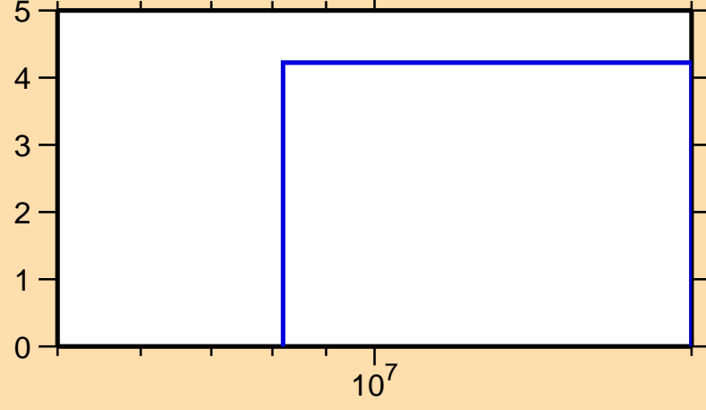
\Delta\sigma/\sigma vs. E for ^{99}\text{In}(n,\text{tot.})
