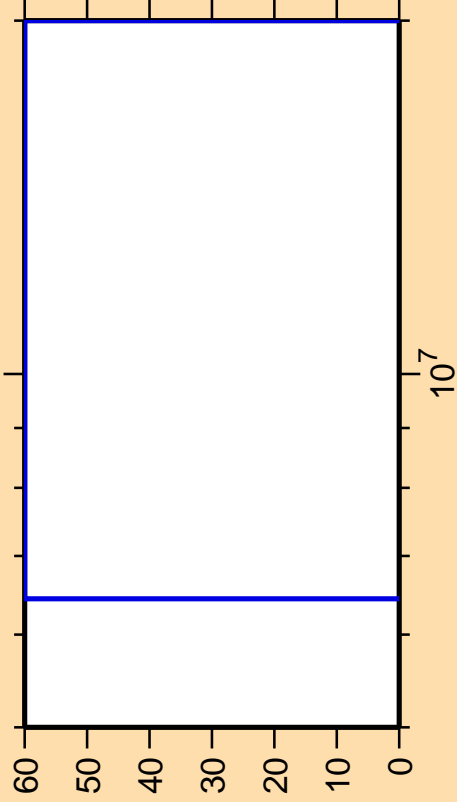
\Delta\sigma/\sigma vs. E for ^{99}\text{In}(n,\text{pd})
