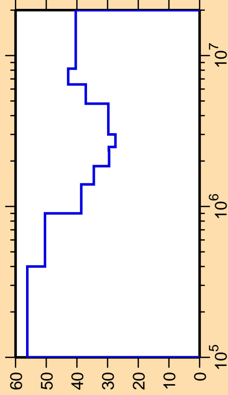
\Delta\sigma/\sigma vs. E for ^{99}\text{In}(n,\text{inel.})
