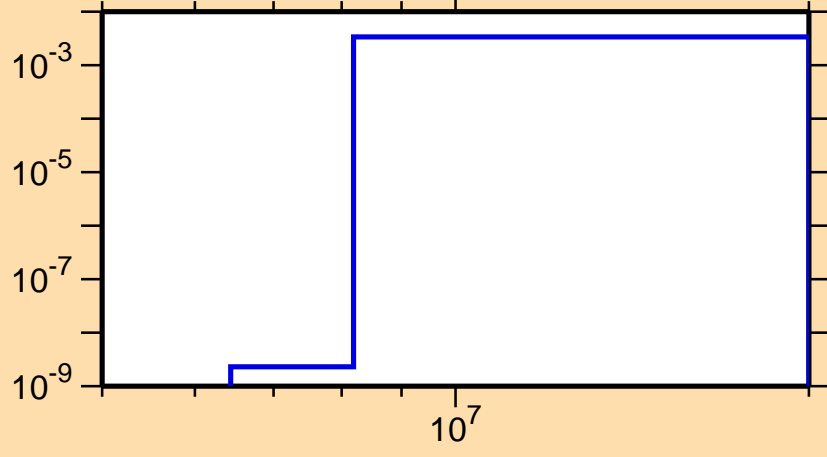
\sigma vs. E for ^{99}\text{In}(n,\text{pd})
