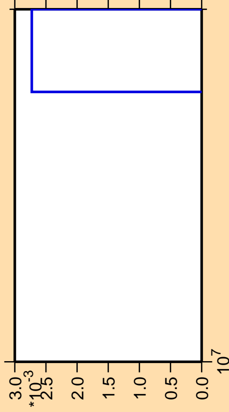
\Delta\sigma/\sigma vs. E for ^{100}\text{In}(n,nt)
