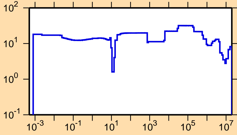
\Delta\sigma/\sigma vs. E for ^{100}\text{In}(n,\text{tot.})
