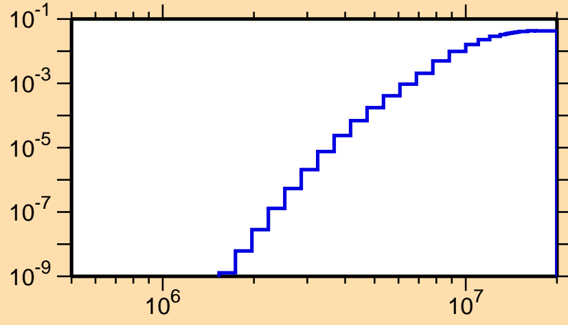
\sigma vs. E for ^{100}\text{In}(n,d)
