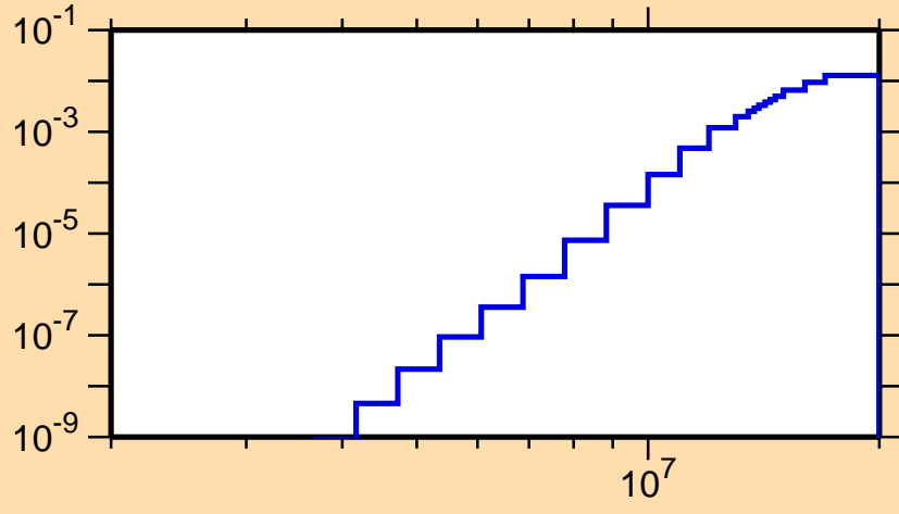
\sigma vs. E for ^{100}\text{In}(n,\text{He}3)
