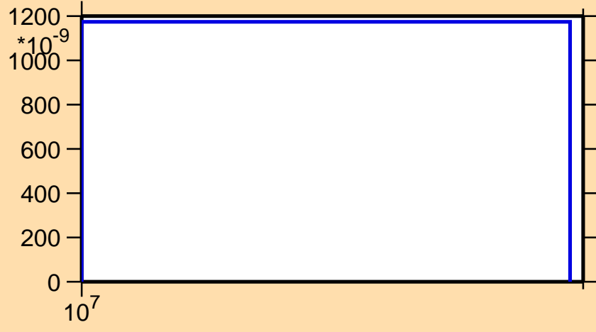
\sigma vs. E for ^{100}\text{In}(n,\text{nd})
