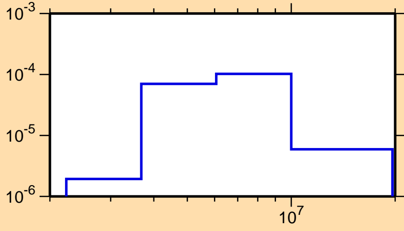
\sigma vs. E for ^{100}\text{In}(n,n_3)
