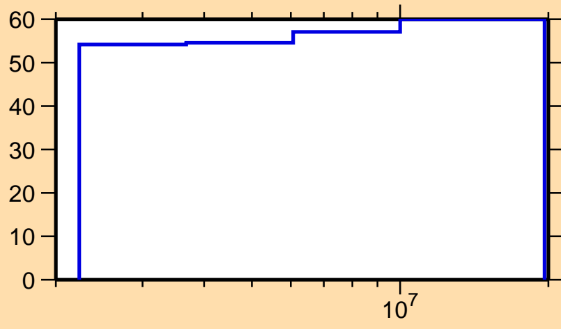
\Delta\sigma/\sigma vs. E for ^{100}\text{In}(n,n_1)
