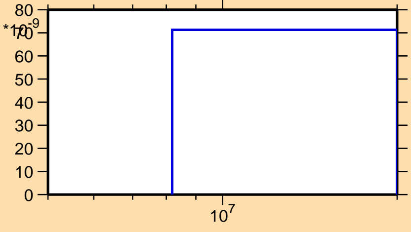
\sigma vs. E for ^{100}\text{In}(\text{mt } 45)
