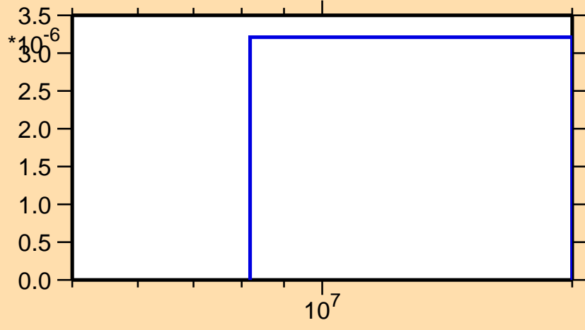
\sigma vs. E for ^{100}\text{In}(n,2np)
