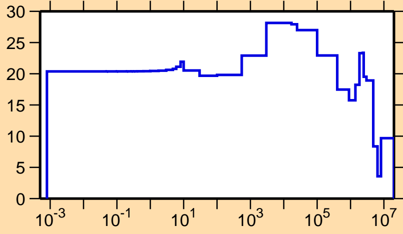
\Delta\sigma/\sigma vs. E for ^{100}\text{In}(n,\text{el.})
