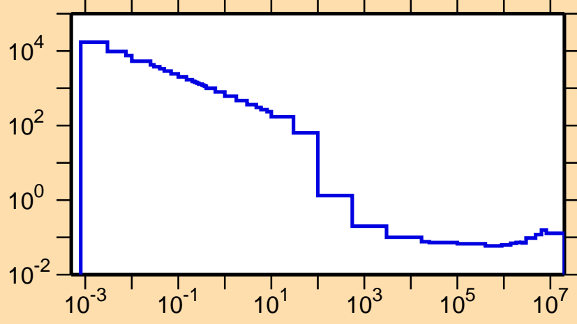
\sigma vs. E for ^{100}\text{In}(n,\alpha)
