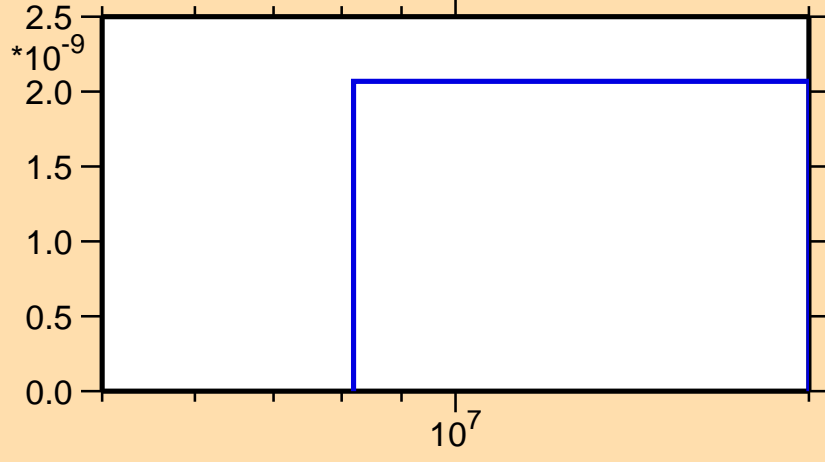
\sigma vs. E for ^{100}\text{In}(\text{mt } 34)
