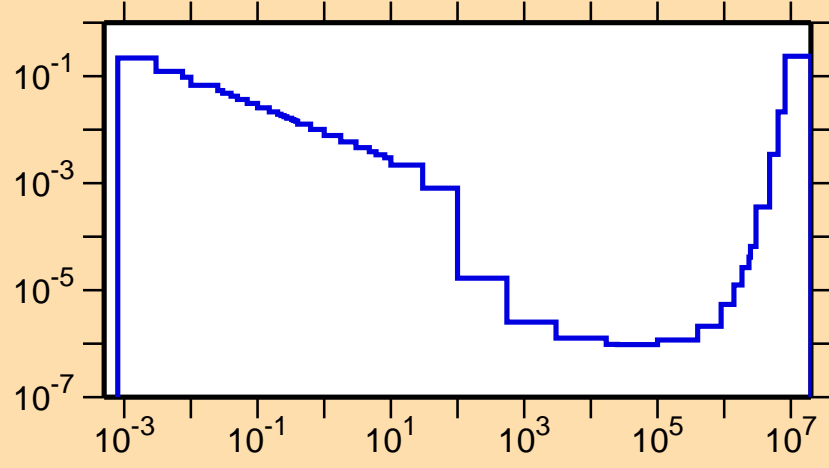
\sigma vs. E for ^{100}\text{In}(n,p)\alpha
