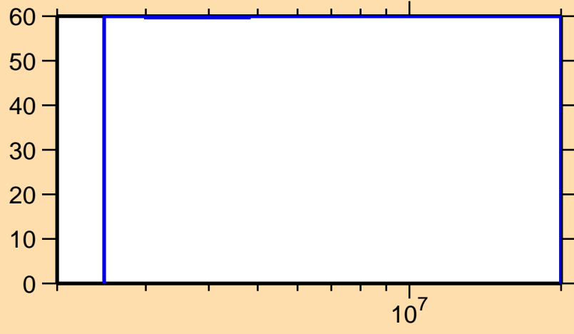
\Delta\sigma/\sigma vs. E for ^{100}\text{In}(n,n\text{cont.})
