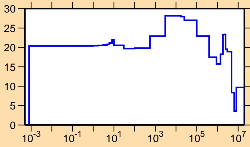
\Delta\sigma/\sigma vs. E for ^{100}\text{In}(n,\text{el.})
