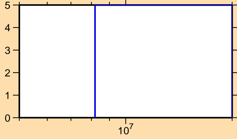
\Delta\sigma/\sigma vs. E for ^{100}\text{In}(n,\text{nonel.})
