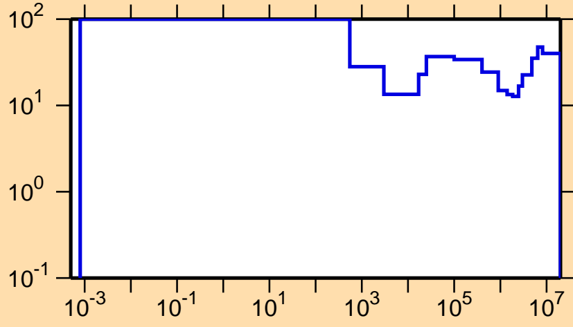
\Delta\sigma/\sigma vs. E for ^{100}\text{In}(n,p)
