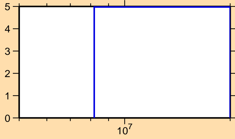
\Delta\sigma/\sigma vs. E for ^{100}\text{In}(n,\text{tot.})
