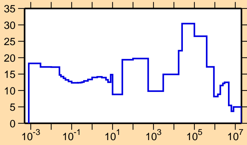
\Delta\sigma/\sigma vs. E for ^{100}\text{In}(n,\text{tot.})
