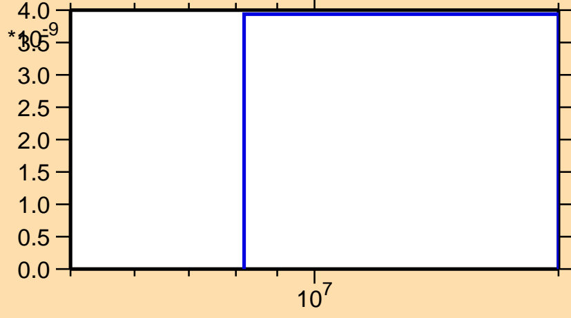
\sigma vs. E for ^{100}\text{In}(\text{mt117})
