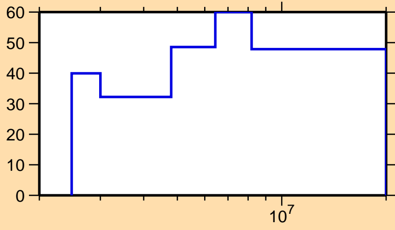
\Delta\sigma/\sigma vs. E for ^{100}\text{In}(n,\text{inel.})
