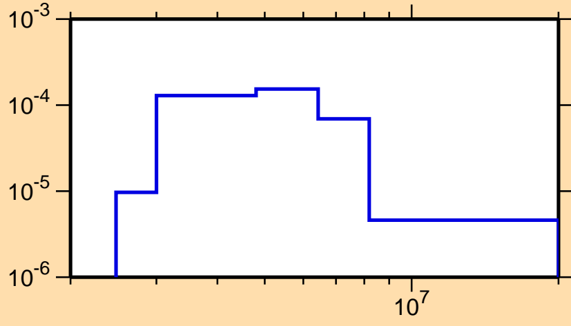
\sigma vs. E for ^{100}\text{In}(n,n_1)
