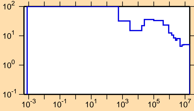
\Delta\sigma/\sigma vs. E for ^{100}\text{In}(n,\text{nonel.})
