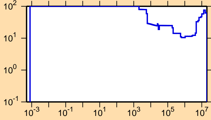
\Delta\sigma/\sigma vs. E for ^{101}\text{In}(n,p)
