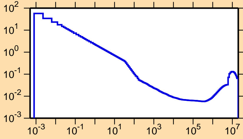
\sigma vs. E for ^{101}\text{In}(n,\alpha)
