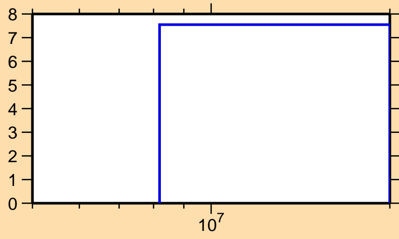
\Delta\sigma/\sigma vs. E for ^{101}\text{In}(n,\text{tot.})
