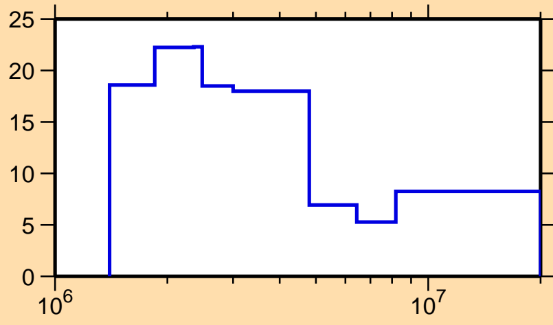
\Delta\sigma/\sigma vs. E for ^{101}\text{In}(n, el.)
