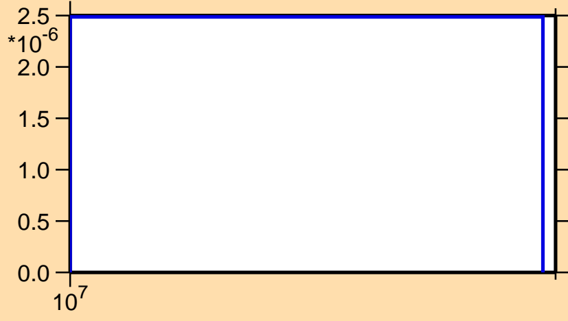
\sigma vs. E for ^{102}\text{In}(n,\text{nd})
