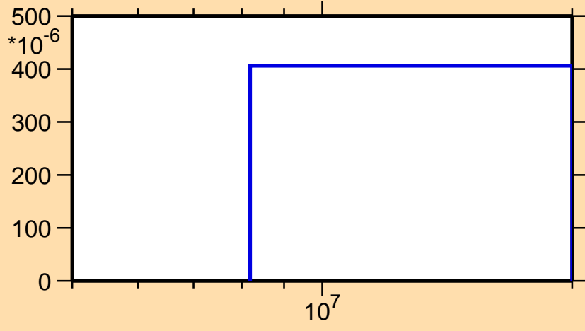
\sigma vs. E for ^{102}\text{In}(n,\text{pd})
