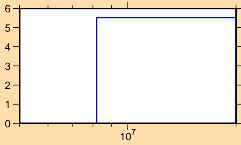
\Delta\sigma/\sigma vs. E for ^{102}\text{In}(n,\text{tot.})
