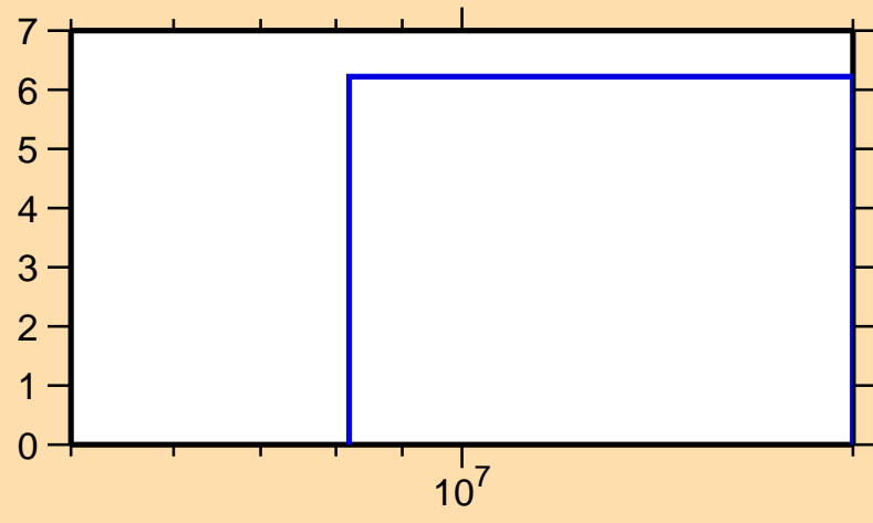
\Delta\sigma/\sigma vs. E for ^{102}\text{In}(n,\text{nonel.})
