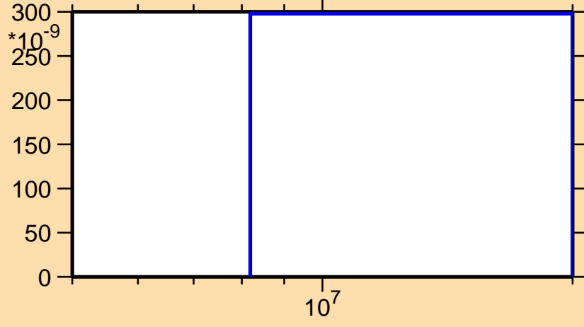
\sigma vs. E for ^{102}\text{In}(\text{mt117})
