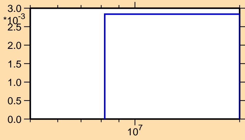
\sigma vs. E for ^{102}\text{In}(n,2n)
