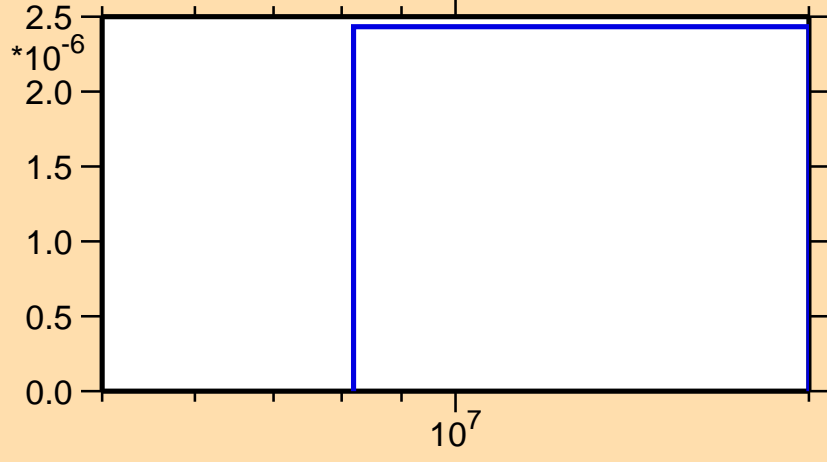
\sigma vs. E for ^{102}\text{In}(\text{mt } 45)
