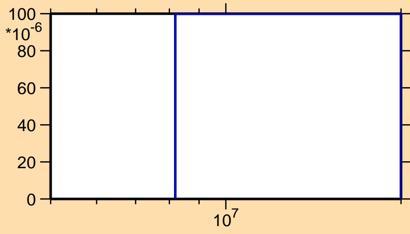
\sigma vs. E for ^{103}\text{In}(n,\text{pd})
