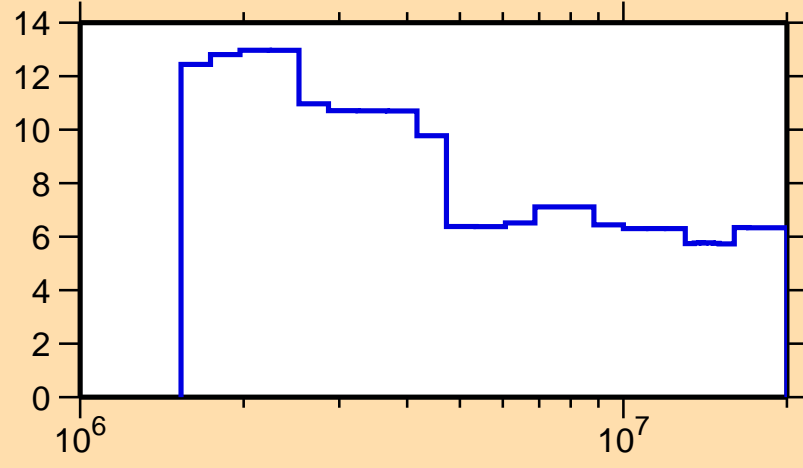
\Delta\sigma/\sigma vs. E for ^{103}\text{In}(n, n_{\text{nonel}})
