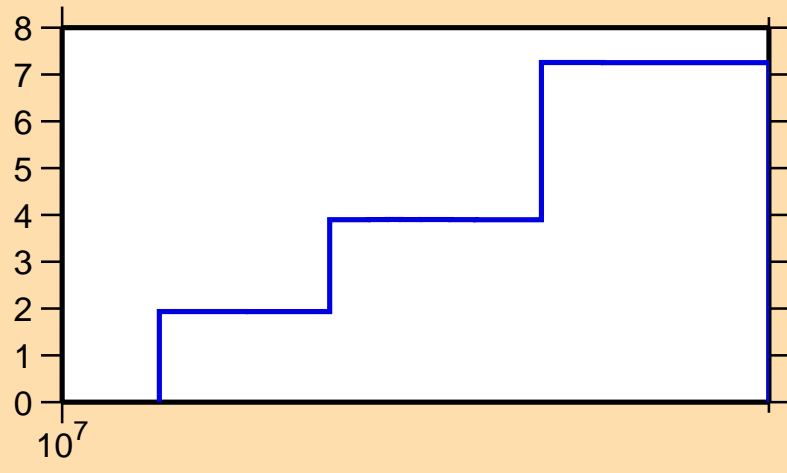
\Delta\sigma/\sigma vs. E for ^{103}\text{In}(n,\text{tot.})
