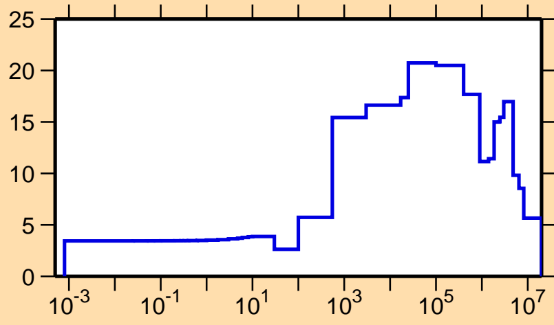
\Delta\sigma/\sigma vs. E for ^{103}\text{In}(n,el.)
