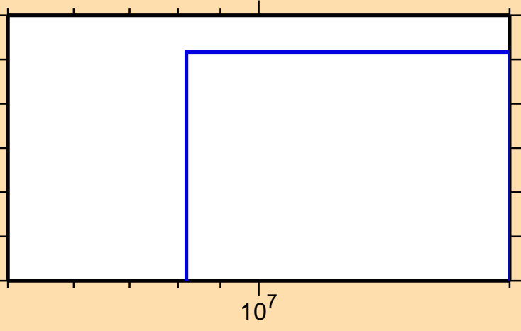
\sigma vs. E for ^{103}\text{In}(n,2np)
